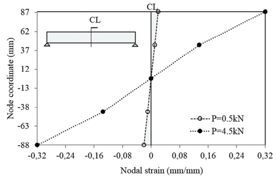
Fig. 7. Nodal strains in the X-X direction
