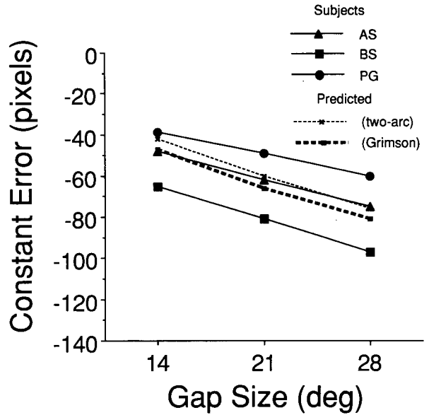
Figure 5. Constant error as a function of gap size for 3 subjects in Experiment 1. See text for explanation of gap size. (Dashed lines show predicted values; see text.)
