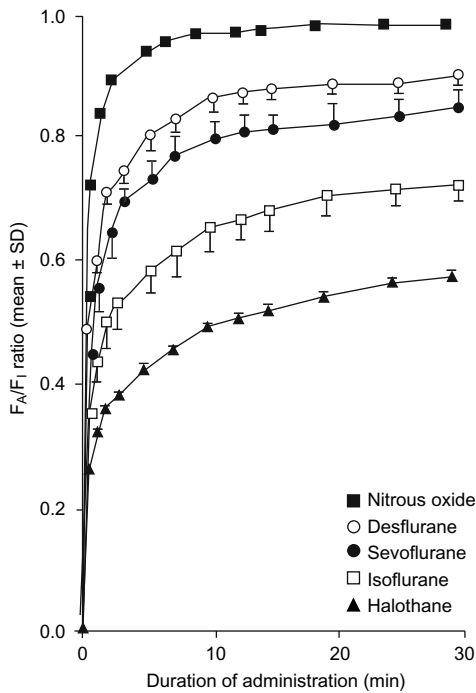
Fig. 4. Pharmacokinetics of sevoflurane during the wash-in phase compared with other inhalational anaesthetics. F_A/F_I is the ratio of end-tidal concentration ( F_A ) to inspired concentration ( F_I ) [from Yasuda et al., [55] with permission].
