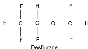
Fig. 1. The chemical structure of some inhalational anaesthetics.
