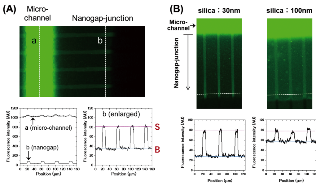
Fig. 5 Selective transport of target molecules into the nanogap-junction formed with silica nanoparticles: (A) Mixed solution of CTB (5 \mu\text{g}/\text{mL} ) and BSA-488 (200 \mu\text{g}/\text{mL} ) (both emitting green fluorescence) was introduced into the micro-channel. In the micro-channel, the background fluorescence of BSA was much more intense than the fluorescence from CTB bound on the fluid bilayer. The signal from CTB was more clearly visible in the nanogap-junction due to suppressed background fluorescence from BSA. The pink line with the sign S and the blue line with the sign B represent the levels of the signal and background, respectively. (B) Effect of silica nanoparticle sizes on the suppression of background noise: fluorescence arising from a mixture of BSA and CTB was compared in the nanogap-junction formed with 30 and 100 nm silica nanoparticles. The background fluorescence intensity was more effectively suppressed for 30 nm nanoparticles compared with 100 nm nanoparticles, thus enhancing the S/B ratio. The images were adapted from Tanabe et al. , 2018.
