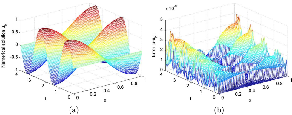
Figure 1. Diagrams of (a) the approximate solution and (b) the associated error up to t = 4 for the (1 + 1)-dimensional hyperbolic problem.
