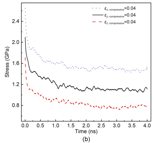
Fig. 5 Change in stress of C-S-H subjected to different uniaxial deformations at T=298 K: (a) evolution of stress under tensile deformation in different directions; (b) evolution of stress under compressive deformation in different directions
