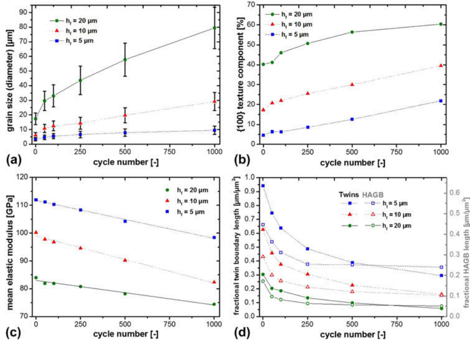
FIG. 2. (a) Grain size evolution of the 5, 10, and 20 \mu\text{m} thick Cu films as a function of cycle number and (b) the corresponding fractional area evolution of the {100} texture component. (c) Evolution of the mean elastic modulus determined from EBSD images. (d) Fractional twin/HAGB evolution with respect to the cycling state.
