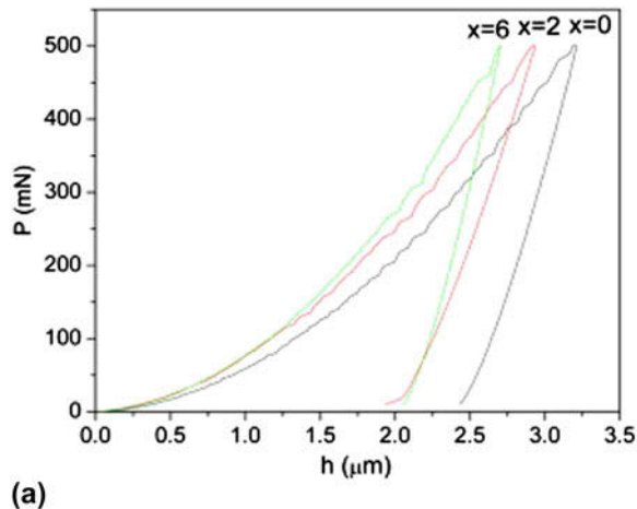
FIG. 8. (a) ( P - h ) nanoindentation curves of \text{Mg}_{72-x}\text{Zn}_{23}\text{Ca}_5\text{Pdx} ( x = 0, 2 and 6 ) alloys and (b) backscattered SEM image showing some indents made close to the center of the \text{Mg}_{70}\text{Zn}_{23}\text{Ca}_5\text{Pd}_2 .
