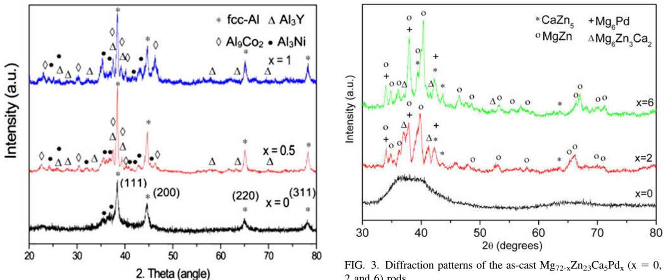
FIG. 2. Diffraction patterns of 1 mm diameter Al_{86}Ni_6Y_{6-x}Co_2Pd_x ( x = 0, 0.5 and 1 ) rods.
