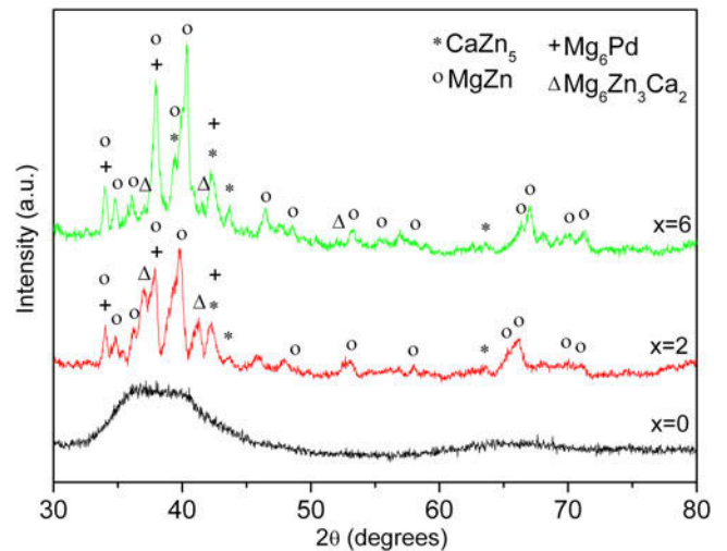
FIG. 3. Diffraction patterns of the as-cast Mg_{72-x}Zn_{23}Ca_5Pd_x ( x = 0, 2 and 6 ) rods.
