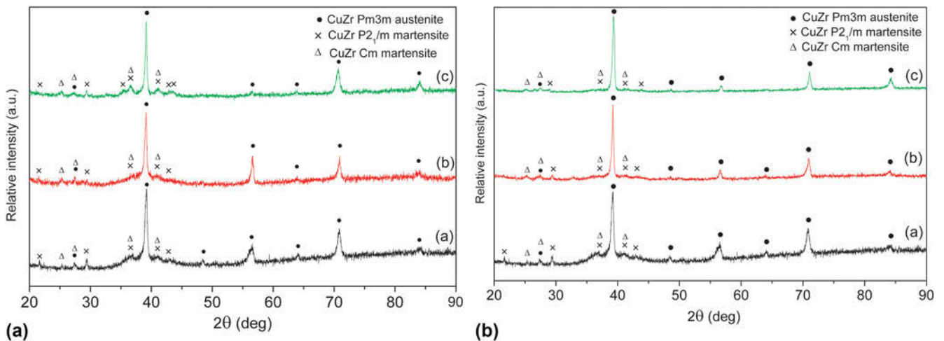
FIG. 1. A) Diffraction patterns corresponding to (a) Zr_{48}Cu_{48}Al_4 , (b) Zr_{48}Cu_{47.5}Al_4Co_{0.5} , and (c) Zr_{48}Cu_{47}Al_4Co_1 as-cast rods. B) Diffraction patterns corresponding to (a) Zr_{48}Cu_{48}Al_4 , (b) Zr_{48}Cu_{47.5}Al_4Fe_{0.5} , and (c) Zr_{48}Cu_{47}Al_4Fe_1 as-cast rods.
