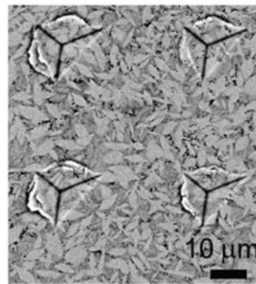
FIG. 8. (a) ( P - h ) nanoindentation curves of \text{Mg}_{72-x}\text{Zn}_{23}\text{Ca}_5\text{Pdx} ( x = 0, 2 and 6 ) alloys and (b) backscattered SEM image showing some indents made close to the center of the \text{Mg}_{70}\text{Zn}_{23}\text{Ca}_5\text{Pd}_2 .
