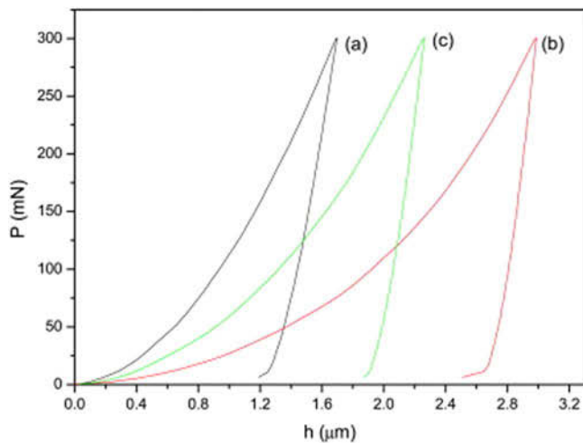
FIG. 7. P - h curves of (a) \text{Al}_{86}\text{Ni}_6\text{Y}_6\text{Co}_2 , (b) \text{Al}_{86}\text{Ni}_6\text{Y}_{5.5}\text{Co}_2\text{Pd}_{0.5} , and (c) \text{Al}_{86}\text{Ni}_6\text{Y}_5\text{Co}_2\text{Pd}_1 . The corresponding table lists the hardness ( H ), reduced elastic modulus ( E_r ), ratio U_{\text{plastic}}/U_{\text{total}} and maximum nanoindentation depth ( h_{\text{max}} ).
