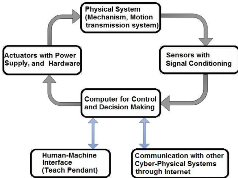
Figure 2: Elements of a typical robotic system.
