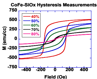
Figure 1. Room temperature hysteresis loops for CoFe nanoparticles dispersed in SiO 2 with volume fractions ranging from 40% to 80% (data are volume normalized and presented in emu/cc).
