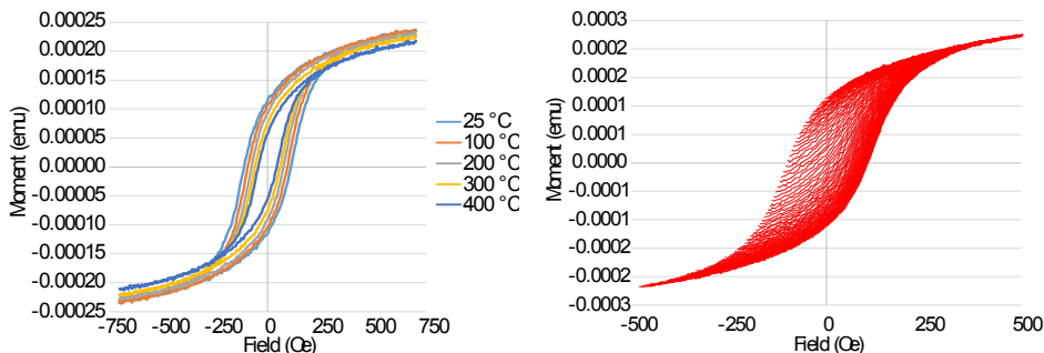
Figure 3. Hysteresis loops at T = 25, 100, 200, 300 and 400\text{ }^{\circ}\text{C} (left) and measured FORCs at 25\text{ }^{\circ}\text{C} (right) for CoFe nanoparticles (40%) dispersed in \text{SiO}_2 (60%).
