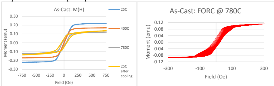
Figure 5. M(H) (left) at 25, 400, 780 and 25 °C after cooling, and the measured FORCs (right) at 780 °C for as-cast FeCo-based nanocrystalline amorphous/nanocomposite sample.
