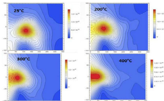
Figure 4. 2D FORC diagrams at T = 25, 200, 300 and 400\text{ }^{\circ}\text{C} .
