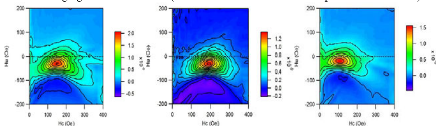
Figure 2. Room temperature 2D FORC diagrams for CoFe nanoparticles dispersed in SiO 2 volume fractions of 40% (left), 50% (middle) and 60% (right).
