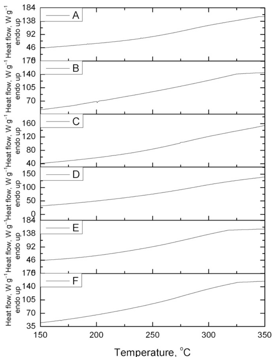
Fig. 12. Glass transition temperatures deduced from DSC curves for material: PI-zeolite-5.2 mass % PDMS ( 3200 \text{ g mol}^{-1} ) (A), PI-zeolite-3.2 mass % PDMS ( 3200 \text{ g mol}^{-1} ) (B), PI-zeolite-5.2 mass % PDMS ( 1000 \text{ g mol}^{-1} ) (C), PI-zeolite-3.2 mass % PDMS ( 1000 \text{ g mol}^{-1} ) (D), PI-zeolite (E), and PI (F).
