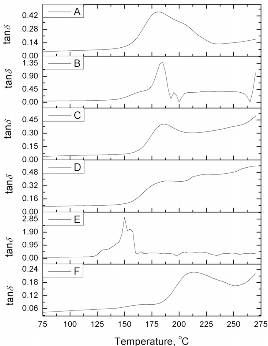
Fig. 13. Glass transition temperatures deduced from DMA for material: PI-zeolite-5.2 mass % PDMS (3200 g mol -1 ) (A), PI-zeolite-3.2 mass % PDMS (3200 g mol -1 ) (B), PI-zeolite-5.2 mass % PDMS (1000 g mol -1 ) (C), PI-zeolite-3.2 mass % PDMS (1000 g mol -1 ) (D), PI-zeolite (E), and PI (F).
