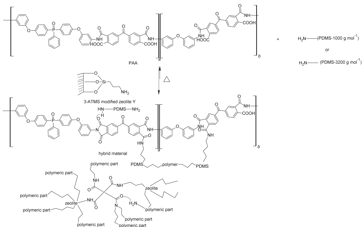
Fig. 1. PI-zeolite-PDMS hybrid material.
