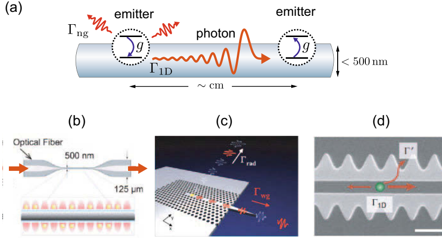
Fig. 13. – (a) Sketch of a waveguide QED setup with two quantum emitters coupled to a 1D photonic channel. If the rate of emission into the waveguide, \Gamma_{1D} , exceeds the emission rate \Gamma_{ng} into other, non-guided modes, efficient long-range interactions between multiple emitters can be attained. This 1D regime of light-matter interactions can be implemented, for example, with (b) trapped atoms coupled to the evanescent field of a tapered nanofiber (reprinted fig. 1 with permission from ref. [174]. Copyright (2011) by the American Physical Society), (c) QDs coupled to a photonic-crystal waveguide (reprinted fig. 1a with permission from ref. [175]. Copyright (2014) by the American Physical Society), or (d) by combining cold atoms and nanophotonic crystal structures in a so-called alligator waveguide setup (reprinted fig. 1a with permission from ref. [176]. Copyright (2014) by the Springer Nature Publishing Group).
