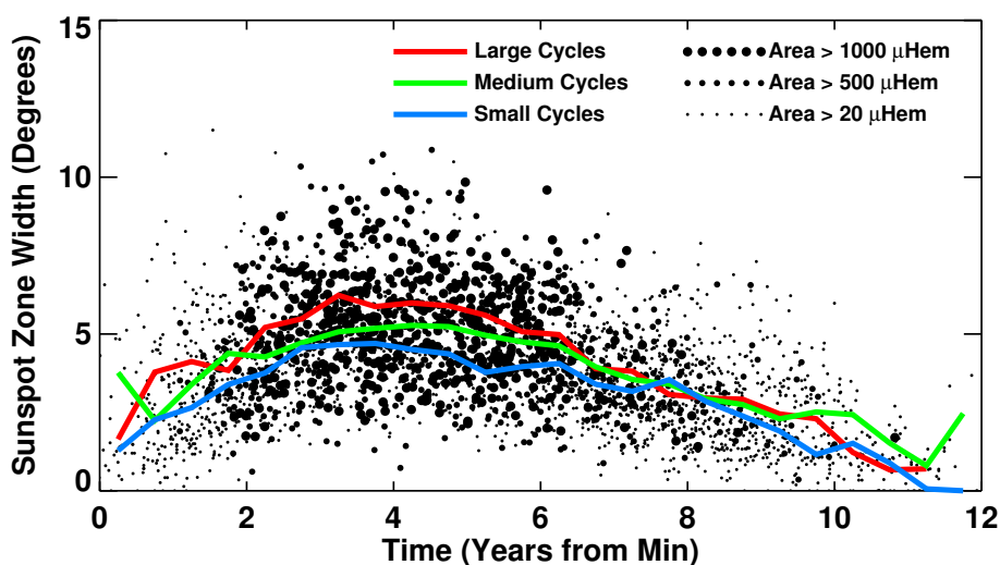
Figure 29: Latitudinal widths of the sunspot area centroid in each hemisphere for each Carrington Rotation as functions of time from cycle minimum. Three symbol sizes are used to differentiate data according to the daily average of the sunspot area for each hemisphere and rotation. The centroids of the centroids in 6-month intervals are shown with the red line for large amplitude cycles, with the green line for medium amplitude cycles, and with the blue line for the small amplitude cycles.
