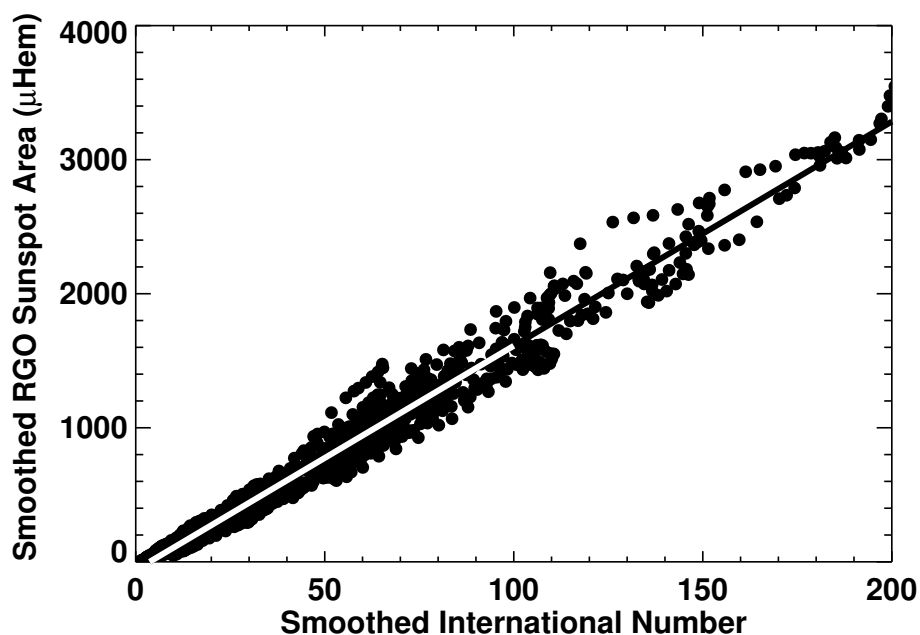
Figure 6: RGO Sunspot Area vs. the International Sunspot Number at monthly intervals from 1997 to 2010. The two quantities are correlated at the 99.4% level with a proportionality constant of about 16.7.
