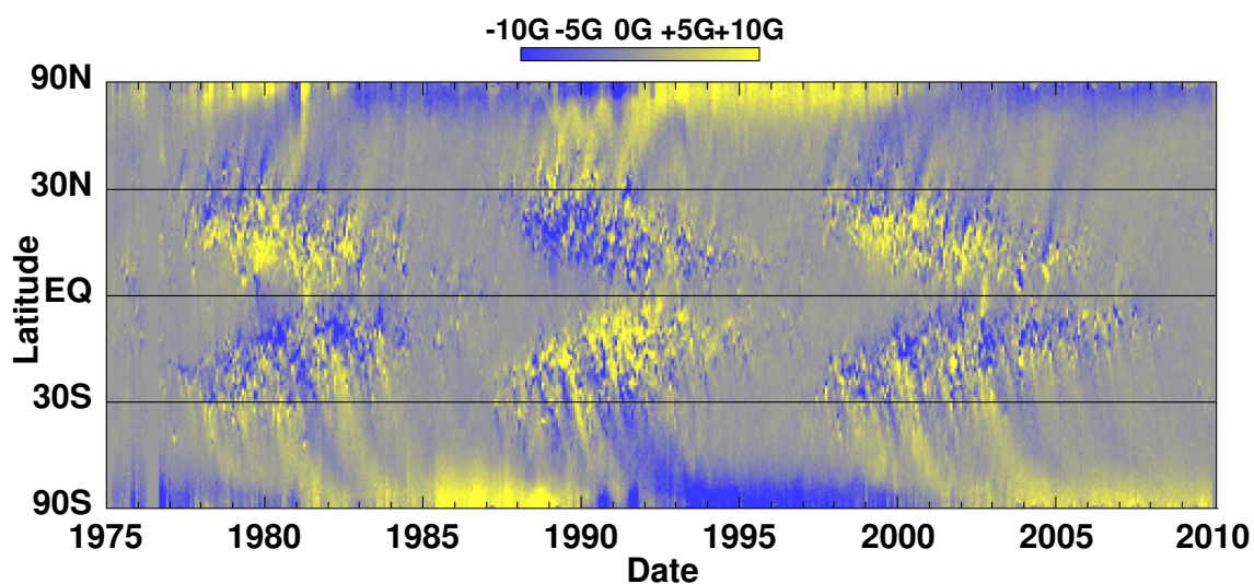
Figure 14: A Magnetic Butterfly Diagram constructed from the longitudinally averaged radial magnetic field obtained from instruments on Kitt Peak and SOHO. This illustrates Hale's Polarity Laws, Joy's Law, polar field reversals, and the transport of higher latitude magnetic field elements toward the poles.
