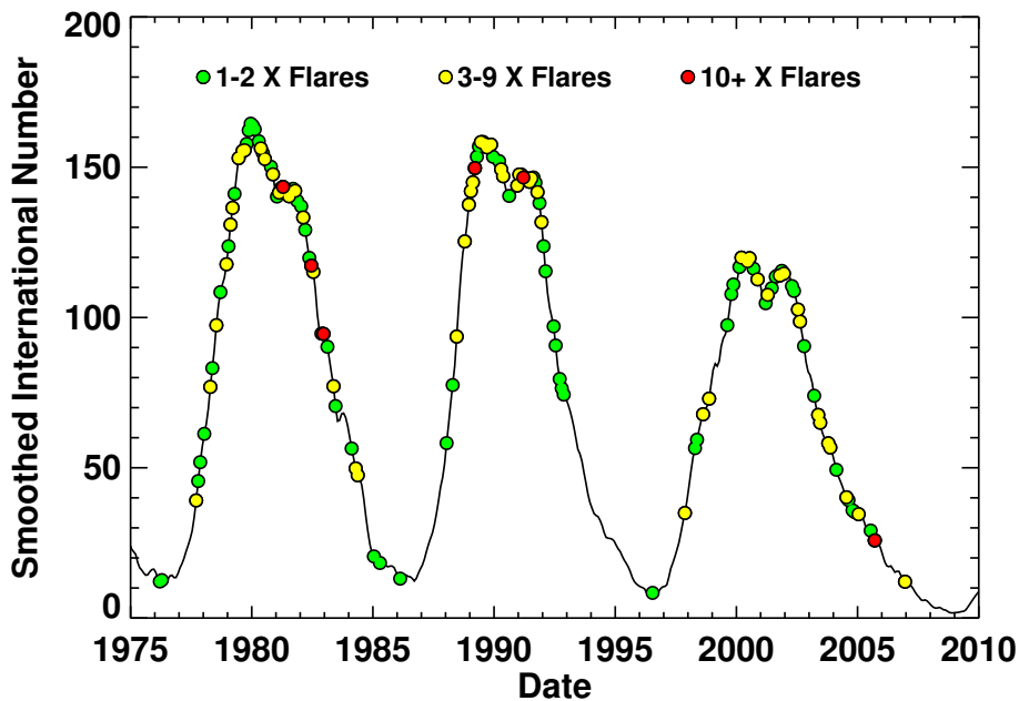
Figure 16: Monthly X-class flares and International Sunspot Number. X-class flares can occur at any phase of the sunspot cycle – including cycle minimum.
