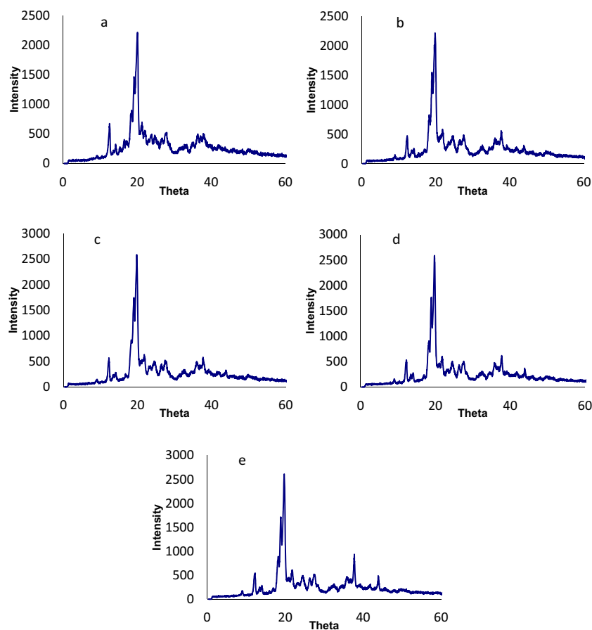
Fig. 6. X-ray powder diffraction profiles of LMH-based proliposomes. a F6. b F7. c F8. d F9. e F10
