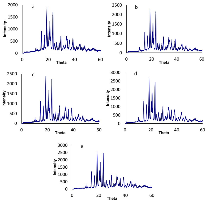
Fig. 4. X-ray powder diffraction profiles of mannitol-based proliposomes. a F1. b F2. c F3. d F4. e F5
