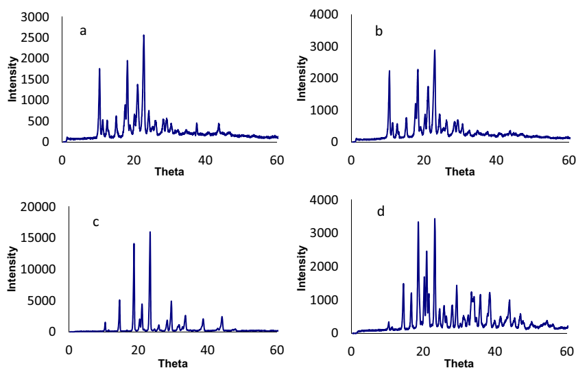
Fig. 3. X-ray powder diffraction of SS (a) and mannitol (c) prior to spray-drying, as well as SS (b) and mannitol (d) after spray-drying in ethanolic suspension
