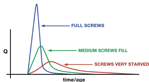
Fig. 13. Effect of the degree of fill on the residence time distribution in a TSE
