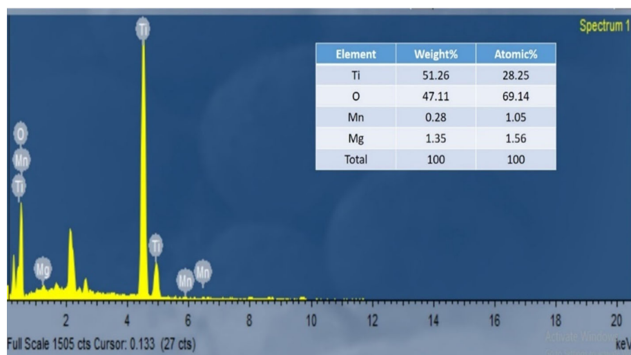
Fig. 5 EDX spectrum of 0.25 wt% Mn^{2+} and 1.00 wt% Mg^{2+} bimetal doped TiO_2 in the presence of 10 wt% of surfactant (MMT5-GS2) after calcination
