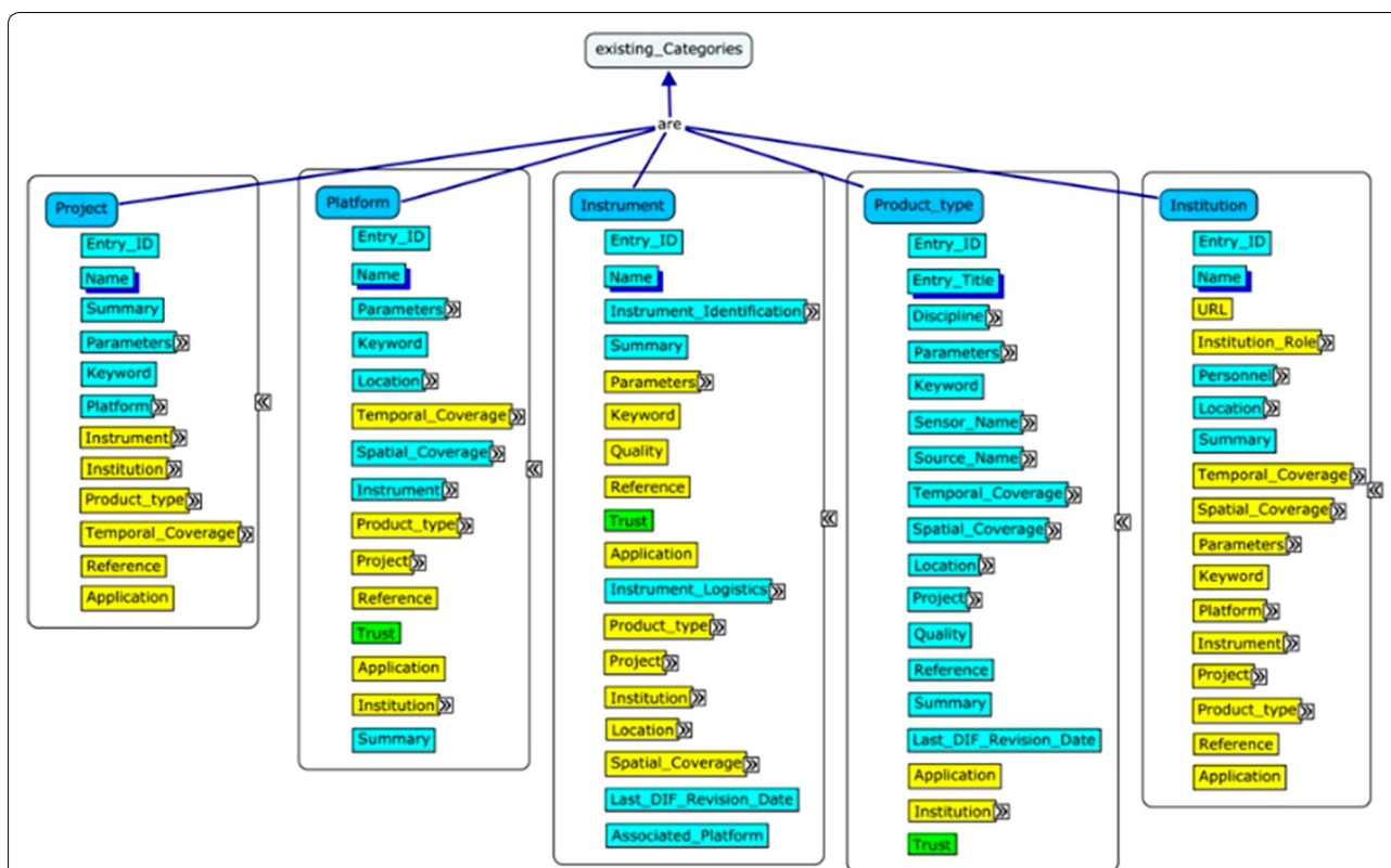
Fig. 2 Main classes and elements of the extended ISDC DIF data model. The cyan colored elements are taken from NASA's DIF standard; the yellow and green colored one are ISDC extensions to this standard. The figure is taken from Sabine Pfeiffer's Master of Engineering Thesis (Pfeiffer 2010)
