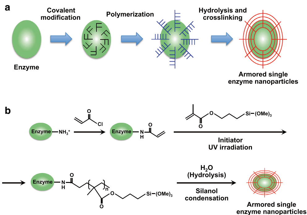
Fig. 9 Illustration of armored single-enzyme nanoparticles. a Schematic of preparation of the single-enzyme nanoparticles. b Chemistry for the synthesis of single-enzyme nanoparticles (Figure adapted with permission from Ref. [90]. Copyright (2003) American Chemical Society)
