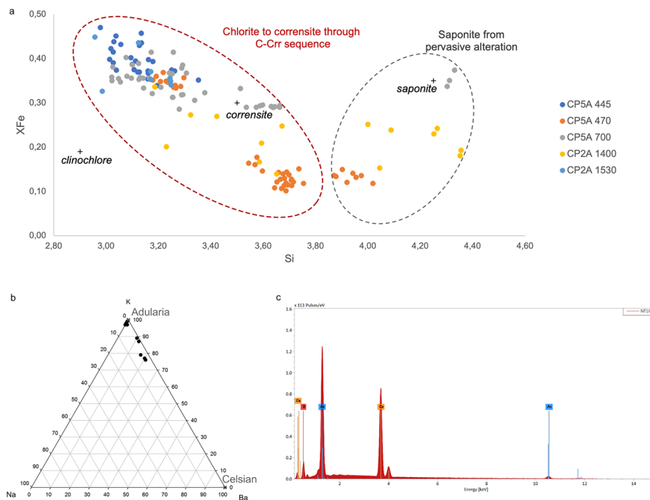
Fig. 7 a Plot of structural formulae of trioctahedral clays in a diagram of XFe versus Si for CP5A and CP2A wells ( XFe = Fe/(Fe + Mg) ). The average structural formulae are presented in Additional file 1: Tables S1, S2, S3. In this figure all the samples are represented with a relative structure containing 14 oxygen atoms and assuming that the total iron content was composed of Fe2+. Theoretical compositions of clinocllore, corrensite, and saponite are provided for reference. b Chemical compositions of K-rich and Ba-rich feldspars at 445 m depth in CP5A well plotted in a Na–K–Ba ternary diagram. Representative analyses are described in Table 1. Theoretical compositions of adularia and celsian are given for reference (crosses). c representative SEM–EDS spectrum of calcium arsenate mineral observed at 470 m depth in CP5A well
