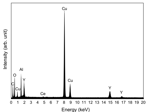
Fig. 3 EDX spectra of nanoparticles (laser energy densities: 3.7 J/cm 2 )
