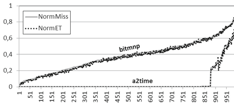
Fig. 7 \text{NormMiss} and \text{NormET} for a2time and bitmnp sorted by \text{NormMiss}
