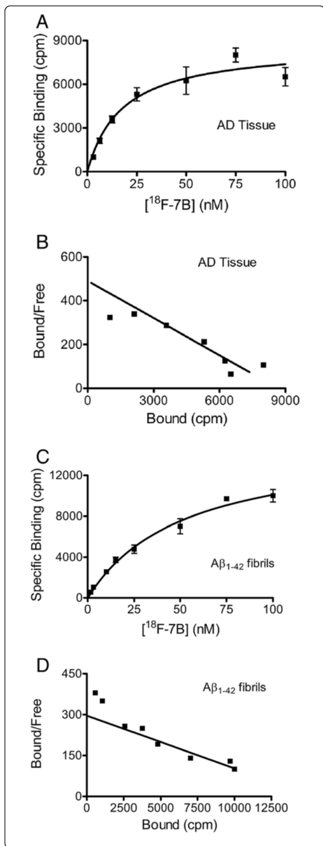
Figure 2 Binding of [ 18 F]-7B with Aβ 1-42 fibrils and AD homogenates. AD homogenates ( A, B ) and Aβ 1-42 fibrils ( C, D ) were incubated with increasing concentrations of [ 18 F]-7B. Nonspecific binding was determined in parallel experiments utilizing 7A (5 μM) as a competitor. Representative plots of specific binding versus [ 18 F]-7B concentration are shown for AD homogenates in ( A ) and Aβ fibrils in ( C ). Data points represent mean ± standard deviations (n = 3). The data were analyzed by curve fitting to a one-site binding model using a nonlinear regression. Scatchard plots of the binding data are shown for AD homogenates ( B ) and Aβ 1-42 fibrils ( D ). Similar results were obtained in more than three independent experiments.
