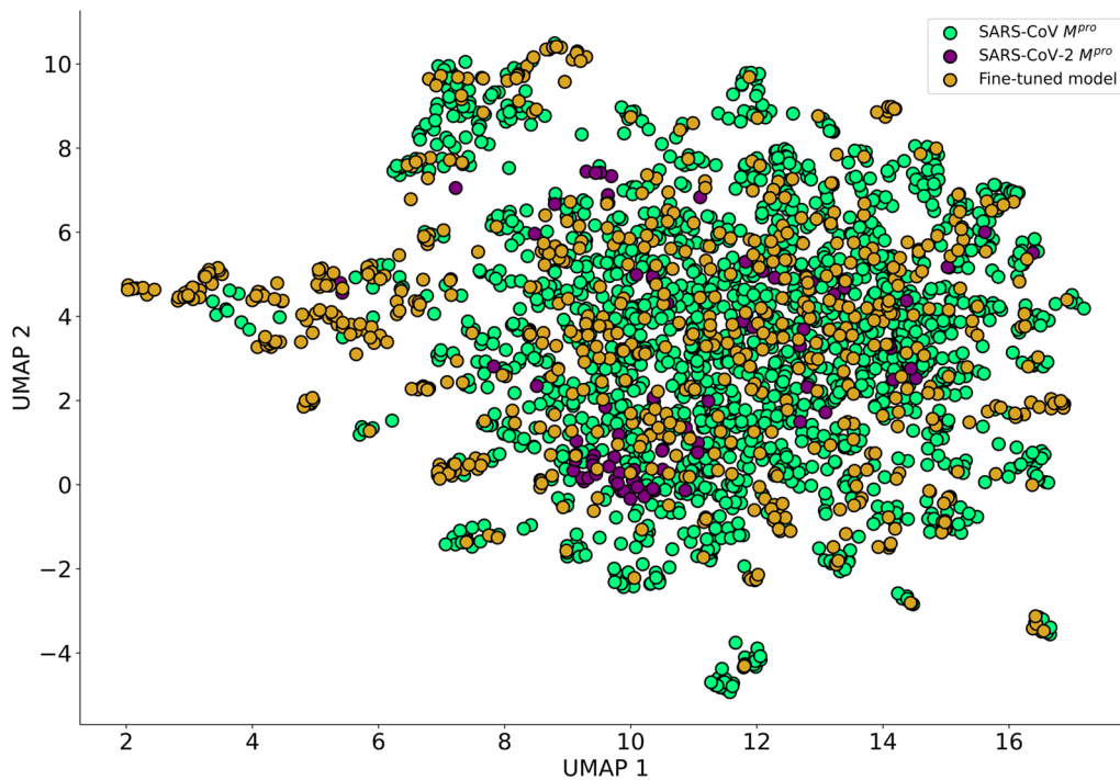
Fig. 12 Chemical space of predicted hits (yellow) and M^{pro} inhibitors of SARS-CoV-1 (indigo) and SARS-CoV-2 (light green)
