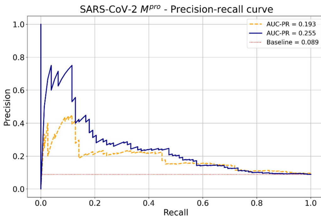
Fig. 11 Precision-recall curves for our model (solid blue line) and chemprop (dashed orange line). The baseline area under the precision-recall curve (AUC-PR) for random predictions is given by the ratio of active molecules in the dataset. For the SARS-CoV-2 M^{pro} , the baseline was 0.089 and is shown as a dotted red line
