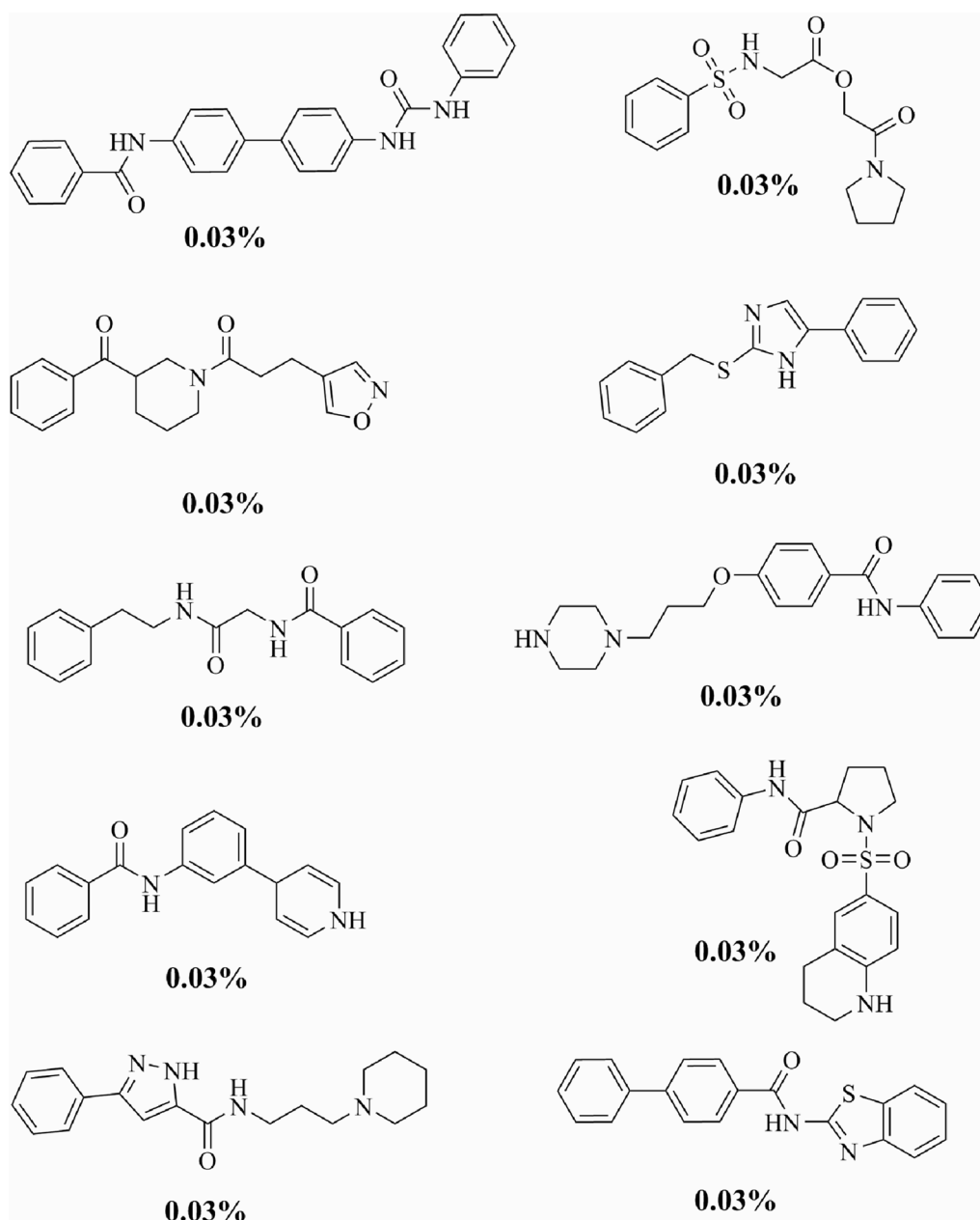
Fig. 5 Top-10 most common novel scaffolds. The prevalence of each scaffold among the generated molecules is also shown
