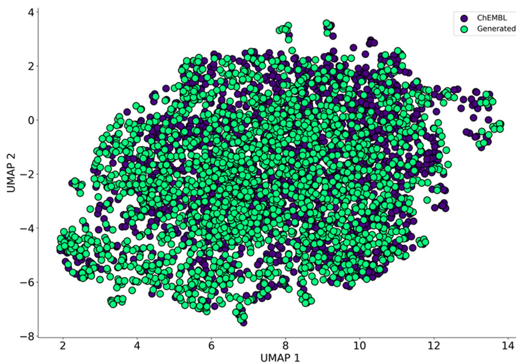
Fig. 3 UMAP plot of the chemical space of molecules generated by the general chemical model and ChEMBL (2000 molecules were randomly selected for each set)
