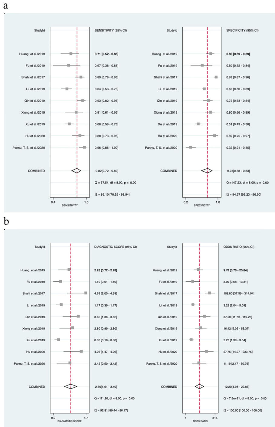
Fig. 4 Forest plot of D-dimer for PJI. a Pooled sensitivity and specificity. b Pooled diagnostic score and diagnostic odds ratio
