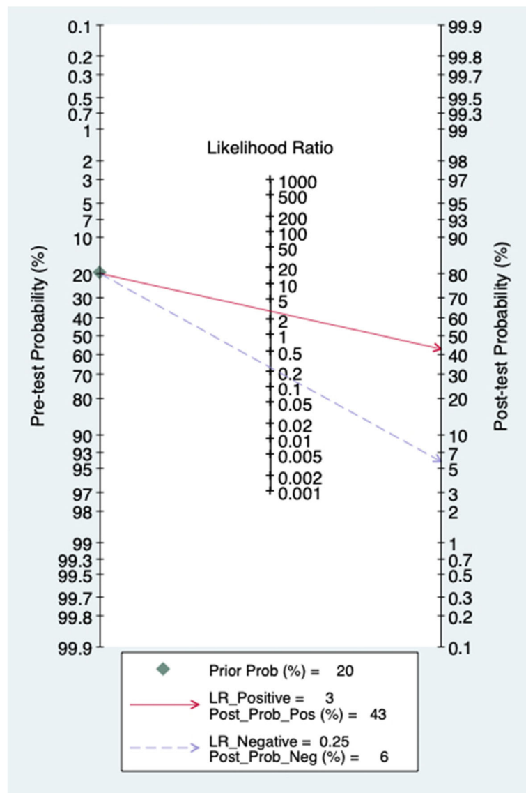
Fig. 7 Fagan's nomogram of the D-dimer for diagnosis of PJI
