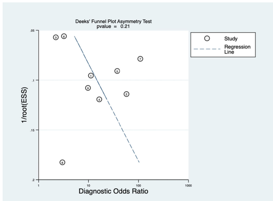
Fig. 3 Funnel plot for publication bias assessment of included studies
