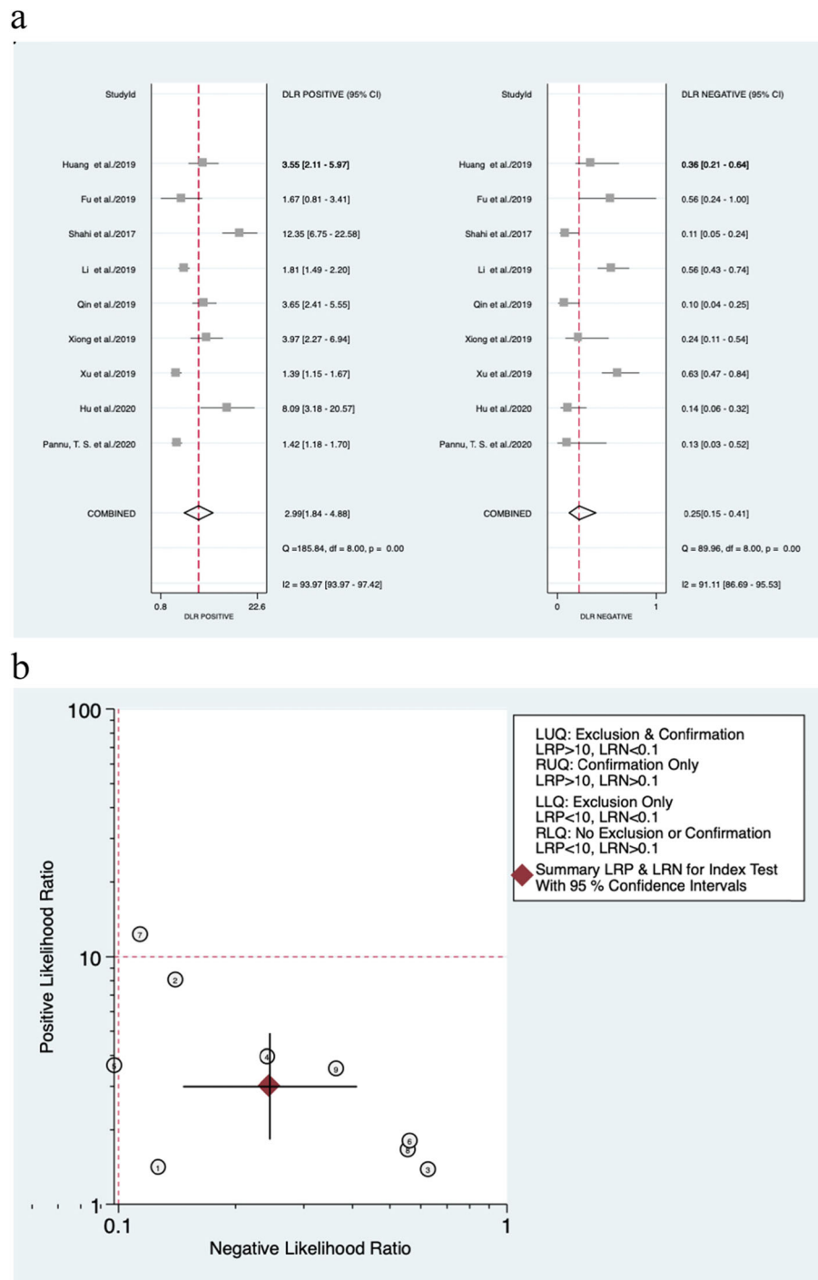
Fig. 6 Forest plots of likelihood ratio (a) and likelihood ratio scatter diagrams (b)
