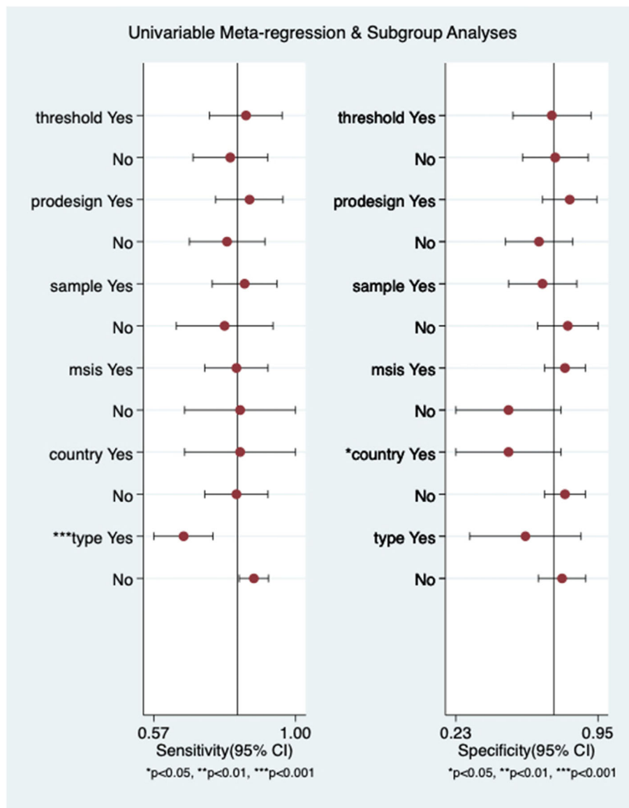
Fig. 8 Meta-regression analysis for D-dimer with several variables
