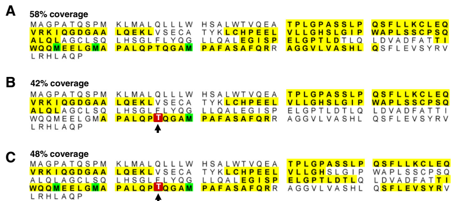
Figure 7 ESI-MS/MS analysis of non-glycosylated and glycosylated Filgrastim™ (G-CSF). (A) Amino acid sequence of the substrate Filgrastim™ showing the tryptic digest peptides detected by ESI-MS/MS (yellow highlight, 58% coverage) and post-translationally modified amino acids (e.g. oxidation, green). G-CSF peptides detected by ESI-MS/MS after treatment with glycosyltransferases (B) HisDapGalNAcT2 (42% coverage) or (C) of rhGalNAcT2 (48% coverage), showing the glycosylation site at Thr 166 (red box and black arrow).
