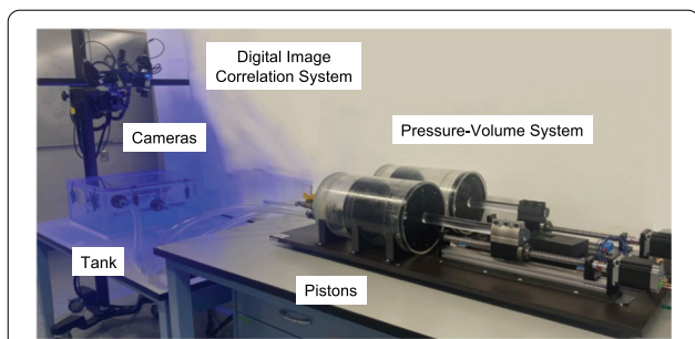
Fig. 1 Experimental set-up of the electromechanical pressure-volume ventilation apparatus (right) interfaced with the digital image correlation system (left). The Trillion ARAMIS Adjustable 12M two-camera system is positioned above a transparent, air-tight tank containing the lung specimen which is controlled by the dual-piston apparatus to apply inflation volumes and measure resulting lung volumes and pressures. The combination of these two systems enables the simultaneous collection of global pressures and volumes and local lung topological strain measurements
