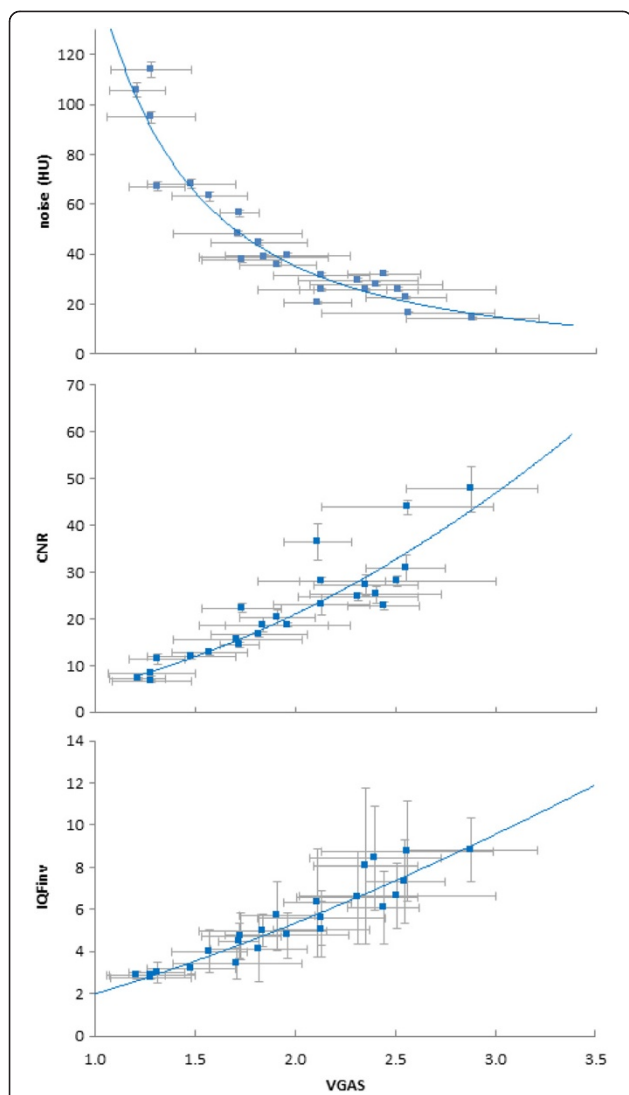
Fig. 3 Mean noise, CNR and IQF inv versus mean VGAS. The error bars in the x direction represent the standard deviation between the scores of the different radiologists. For noise, the error bars in the y direction represent the standard deviation between noise measurements in 11 following slices in the Catphan uniformity module. For CNR, the error bars in the y direction represent the standard deviation between CNR measurements in four consecutive slices of the Catphan CT number linearity and CT number accuracy module. For IQF inv , the error bars in the y direction represent the standard deviation between the six readers of the contrast-detail module in the Catphan phantom. Regression lines were plotted resulting in an r^2 of 0.90, 0.88 and 0.92, p < 0.001 , for noise, CNR and IQF inv respectively
