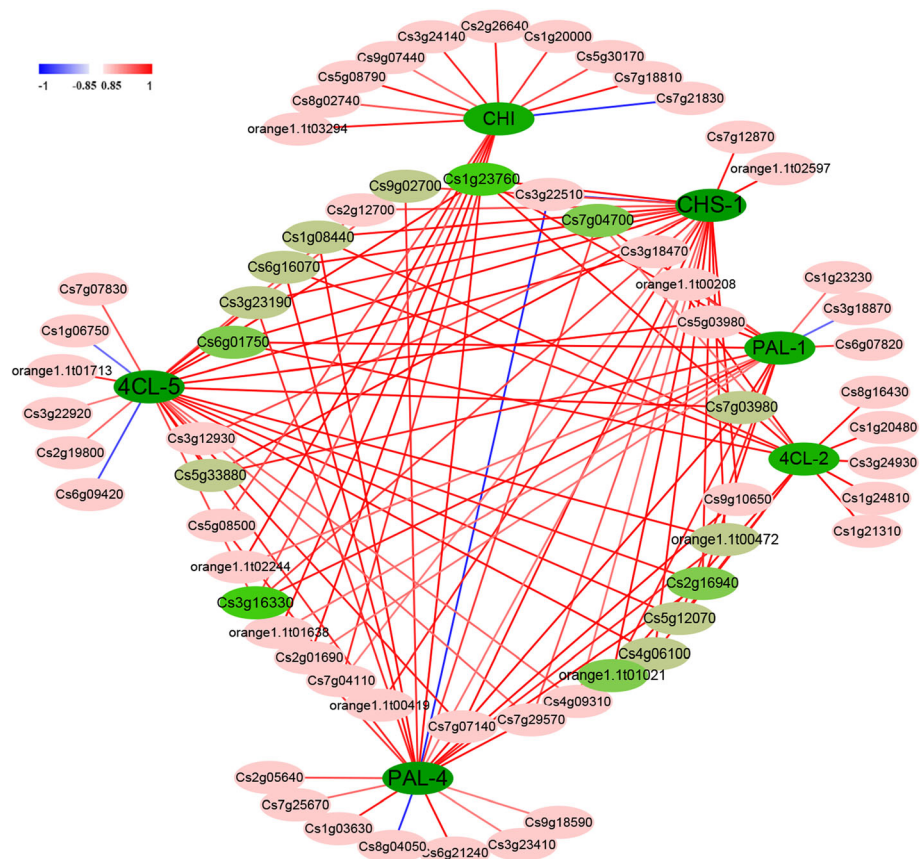
Fig. 6 The relationships between PAL-1 (Cs6g11940), PAL-4 (Cs8g16290), 4CL-2 (Cs5g24900), 4CL-5 (orange1.1104489), CHS-1 (Cs2g14720) and CHI (Cs7g28130) genes and its potential TFs based on transcriptome data
