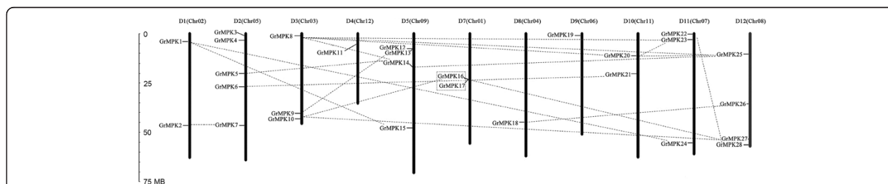
Figure 1 Chromosomal distribution of MAPK genes in G. raimondii . The chromosome numbers are indicated at the top of each bar. The chromosome numbers from D1 to D5, and D7 to D12 were consistent with our newly-updated interspecific genetic map in allotetraploid cultivated cotton species reported recently (Zhao et al. [32]), and the scaffolds name from G. raimondii genome was showed in the bracket. Lines were drawn to connect duplicated genes. The nomenclature of MAPKs were based on the order of the chromosomes in G. raimondii .
