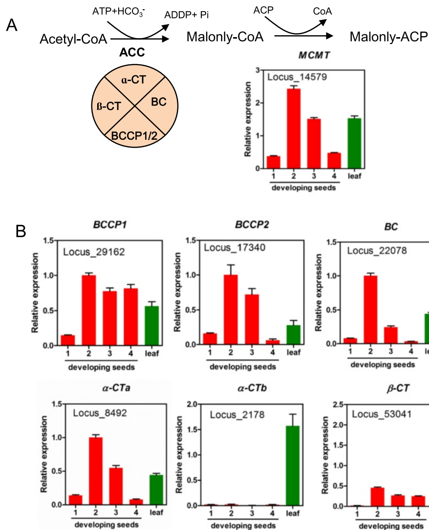
Fig. 4 Synthesis of malonyl-ACP from acetyl-CoA. a Malonyl-ACP synthesis from acetyl-CoA by heteromeric acetyl-CoA carboxylase (Het ACC) and malonyl-CoA:ACP malonyltransferase (MCMT). b Expression of subunits genes of Het ACC complex. Abbreviations are described as in Fig. 2
