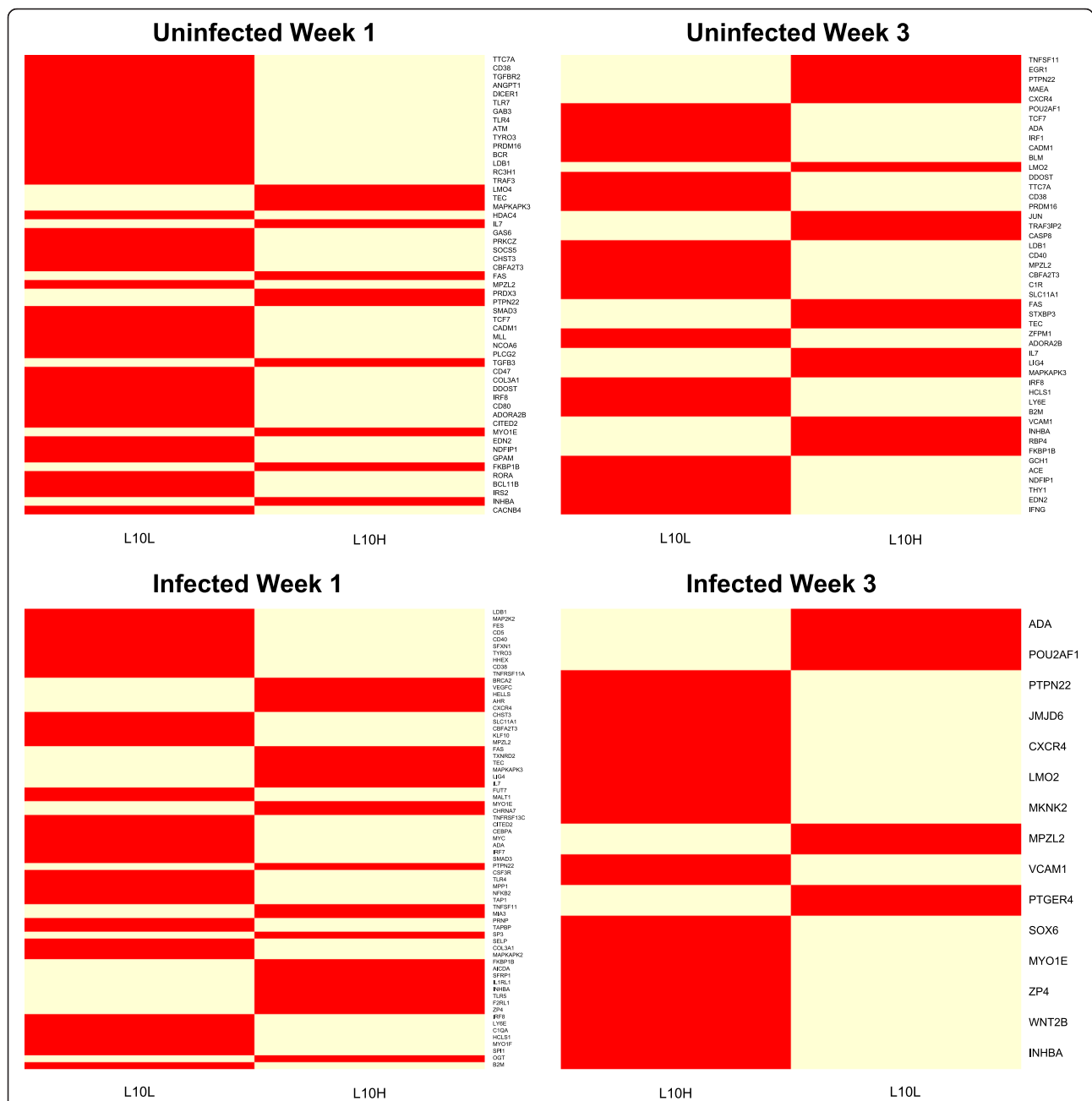
Fig. 4 Differentially expressed genes associated with the GO Immune System term. Heatmap representation of the differentially expressed (DE) genes associated with the GO Immune System terms for the four comparisons between the two lines, L10H and L10L, uninfected and infected groups at two time points, weeks 1 and 3. The heat map is constructed using the average values of counts per millions for each group
