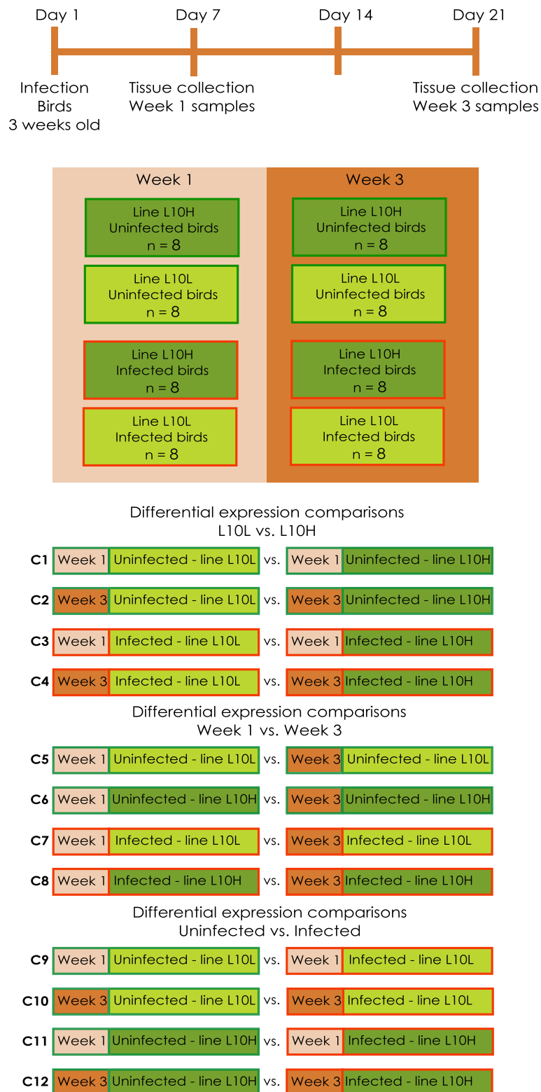
Fig. 1 Structure and timeline of the experiment together with comparisons of gene differential expressions. The figure illustrates the experimental timeline together with the structure of the experiment. In total, 64 birds, 32 from each experimental line, L10H and L10L, were used. In addition, differential expression comparisons are shown
