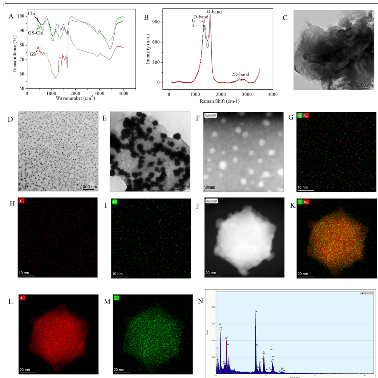
Fig. 2 Characterization of the related nanocomposites. A FT-IR spectra of Chi, GS, and GS-Chi. B Raman spectra of GS (a) and GS-Chi (b). TEM images of GS-Chi ( C ), Chi-Au/Pt ( D ), and GS-Chi-Au/Pt ( E ). HRTEM image of Chi-Au/Pt ( F ). Overlay on the image of Chi-Au/Pt ( G ). Au elemental mapping image of Chi-Au/Pt ( H ). Pt elemental mapping image of Chi-Au/Pt ( I ). HRTEM image of GS-Chi-Au/Pt ( J ). Overlay on an image of GS-Chi-Au/Pt ( K ). Au elemental mapping image of GS-Chi-Au/Pt ( L ). Pt elemental mapping image of GS-Chi-Au/Pt ( M ). EDS elemental analysis of GS-Chi-Au/Pt ( N )
