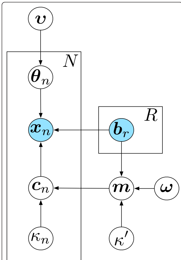
Figure 2 Graphical model representation of the ISOpure model. This directed graph represents the joint probability distribution over the input data (blue circles) and the estimated model parameters (white circles), conditioned on the estimated model hyper-parameters (white circles), in the ISOpure model (equations 3 to 9). The conditional probability of each variable depends only on its parents in the graph. To avoid explicitly representing all N tumor profiles c_n and R normal profiles b_r in the graph (and other associated variables), we used 'plate' notation by drawing one representative node per variable, and enclosing these variables in a plate (rectangular box), where the total number of instances of each enclosed variable is indicated by the fixed constant in the upper right corner of the plate.
