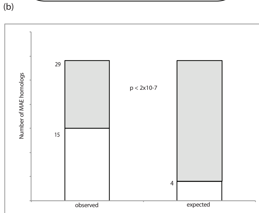
Figure 3 Comparison of random monoallelic expression in human and mouse genomes. (a) Human and mouse random monoallelic expression (RMAE). Of all orthologous gene pairs between mouse and human, there were 529 for which the gene was assessed (as either biallelic expression, RMAE class I or RMAE class II) in each organism. Of these orthologs, 66 were RMAE in mouse and 29 were RMAE in human, resulting in a subset of 15 genes that were assessed as RMAE in both organisms. (b) The number of assessed orthologs showing RMAE in both species is greater than would be expected by chance (Note 6 in Additional file 1). The observed and expected overlaps are shown as subsets of the gray bars, which represent the maximum possible overlap, as defined by the total number of RMAE genes (29) observed in human (for an overlap of 15 or more genes; hypergeometric P < 2 \times 10^{-7} ).
