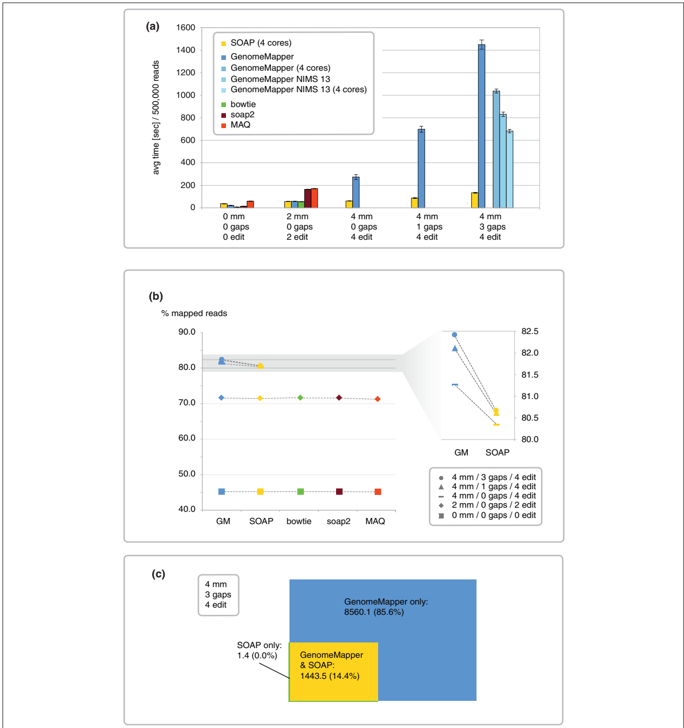
Figure 3 Performance of GenomeMapper compared with that of other short-read alignment tools. (a) Runtime, measured as wall clock time between invocation and termination of the program, averaged from 10 independent tests with different random sets of 500,000 short reads from Est-I. The worst test was excluded from average calculations. Error bars indicate standard deviation. mm , gaps , and edit refer to the maximal number of mismatches, gaps and edit operations allowed. GenomeMapper was run with four different parameter settings: the serial version; the parallel version on four cores; the serial version merely aligning NIMS of length 13 or longer; and the parallel version aligning only NIMS of length 13 or longer. SOAP was found running on up to four CPUs instead of only one CPU, as configured with the command line (option -p). (b) Average sensitivity, measured as the percentage of aligned reads. Only GenomeMapper and SOAP can perform gapped alignments. (c) Average sensitivity of alignments, allowing three gaps and four mismatches with a combined maximum of four edit operations, measured as number of reads with gapped alignments. Fractions refer to the number of all reads with gapped alignments.
