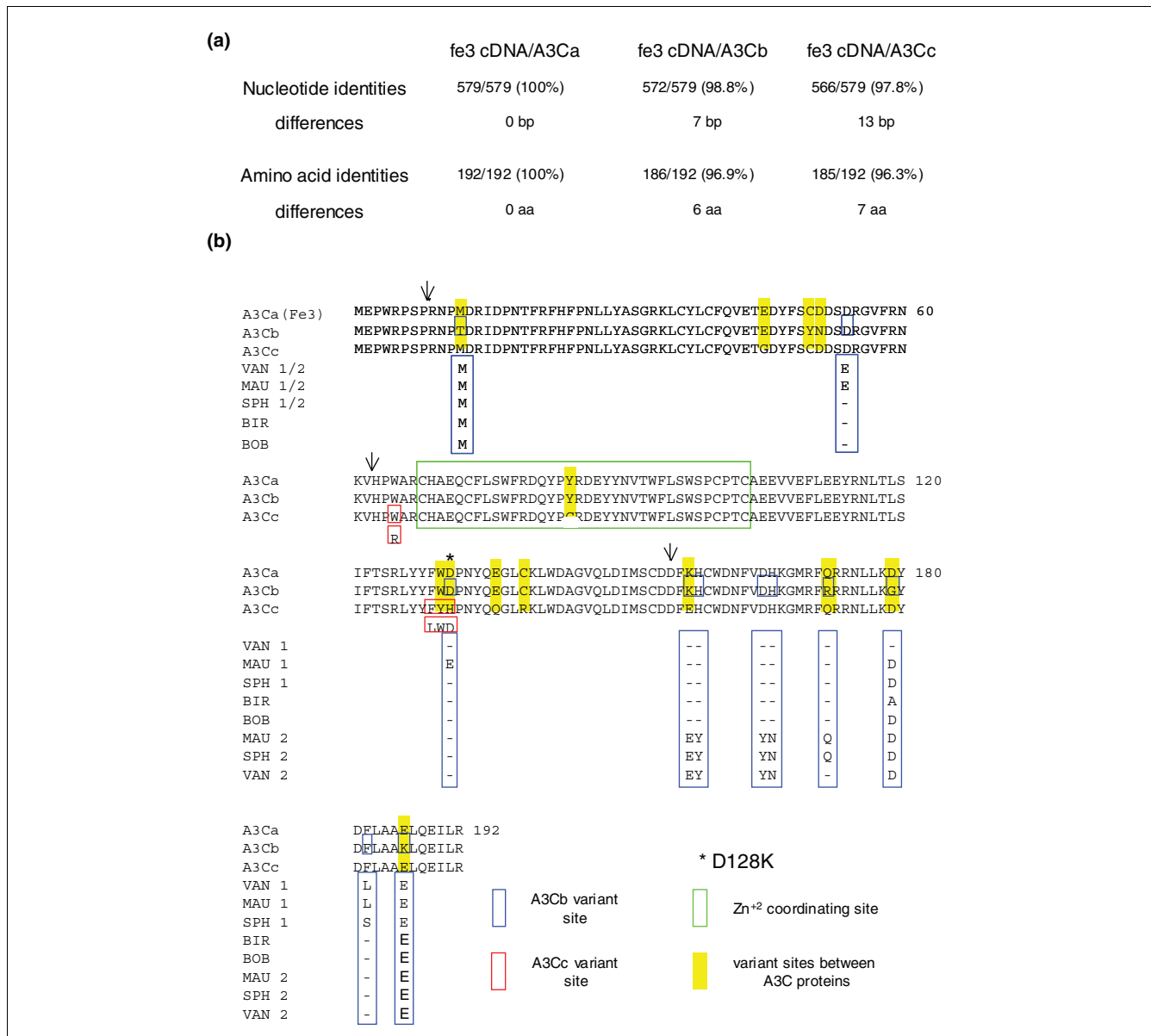
Figure 3 Comparison of the nucleotide coding and amino acid sequences of the feline A3C genes. (a) Pairwise comparison of the domestic cat A3 cDNA to the predicted A3Ca, A3Cb and A3Cc genomic coding sequences and the predicted amino acid sequences. (b) Amino acid sequence alignment of A3C cDNA and the predicted proteins for A3C genes. Highlighted in yellow are amino acid residues different between the A3Cs based on the genomic sequence, whereas amino acid sites displaying non-synonymous amino acid substitutions are boxed in blue and red for A3Cb and A3Cc, respectively, as identified by SNP genotyping of eight domestic cat breeds for exons 2-4 of A3Ca, A3Cb and A3Cc (for more details see Table 4 in Additional data file 2). Arrows indicate exonic junctions. Below the alignments, variant amino acids are boxed in red for A3Cc (for example, W65R) and blue for A3Cb with respect to the breed from which they were identified: Turkish van (VAN), Egyptian mau (MAU), Sphynx (SPH), Birman (BIR) and Japanese bobtail (BOB). A dash indicates the amino acid is identical to genomic sequence. Numbers adjacent to breed identifiers refer to alleles 1 and 2 identified by clonal sequence analysis of the PCR products that are in phase for exons 3 and 4, but not for exon 2 (1/2). The residue corresponding to functionally significant amino acid replacement identified in human A3G (D128K) is highlighted by an asterisk (see text).
