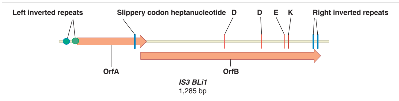
Figure 2 Schematic map of the insertion sequence IS3Bli1 . Nine identical copies of this 1,285-bp element were found in the genome of B. licheniformis ATCC 14580. Features of the IS3Bli1 element are summarized in the text.
