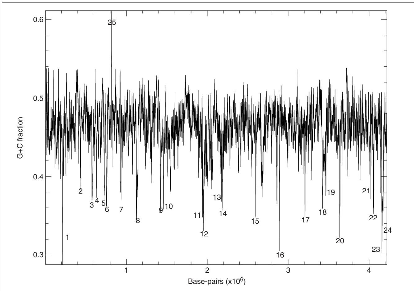
Figure 3 Isochore plot of the B. licheniformis ATCC 14580 genome showing G+C content as a function of position. AT-rich peaks (numbered 1-24) are marked on the plot, and a single island that is atypically GC-rich is indicated by number 25. Table 2 lists the specific chromosomal features represented by each numbered peak.
