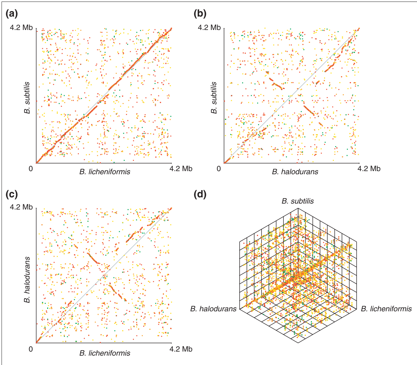
Figure 5 Two- and three-dimensional similarity plots comparing the distribution of orthologs on the chromosomes of B. licheniformis , B. subtilis and B. halodurans . BLAST scores were generated and dots were positioned according to the locations in the genome where orthologs exist in order to view possible regions of possible colinearity. The minimum BLAST expectancy score for each dot in this example was 1 \times 10^{-50} . (a) The plot for B. licheniformis versus B. subtilis ; (b) B. halodurans versus B. subtilis ; (c) B. licheniformis versus B. halodurans ; (d) a three-dimensional scatter plot comparing the distribution of orthologs among all three species. Dots located on the diagonal are indicative of conserved location of orthologous genes between species, whereas a line of dots that lie perpendicular to the diagonal suggests an inversion of a genomic segment between species.
