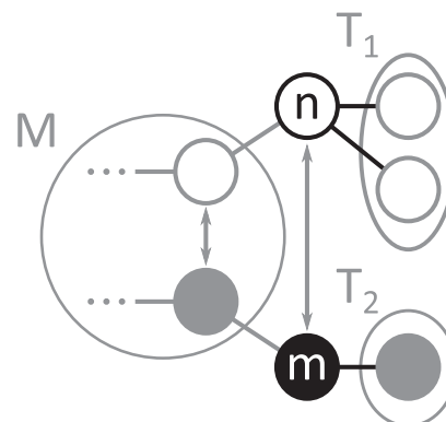
Figure 6 VF2 feasibility rule for node cardinality (1-look-ahead). VF2 feasibility rule for node cardinality (1-look-ahead). The rule prohibits an extension of the current solution M(s) by candidates with a substructure cardinality that can not be fully mapped onto the graph. In the given example, node m has one edge into T_2(s) and is mapped to atom n with a cardinality of two. Therefore, the mapping is feasible.
