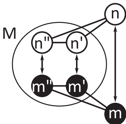
Figure 5 VF2 feasibility rule for node cardinality. VF2 feasibility rule for node cardinality. The rule guarantees a one-to-one mapping of edges in the current solution M(s) . For a candidate mapping (n, m) , all atoms ( n' and n'' in M_1(s) ) adjacent to n must be mapped to the corresponding nodes ( m' and m'' in M_1(s) ) adjacent to m . Otherwise the candidate mapping is not feasible.
