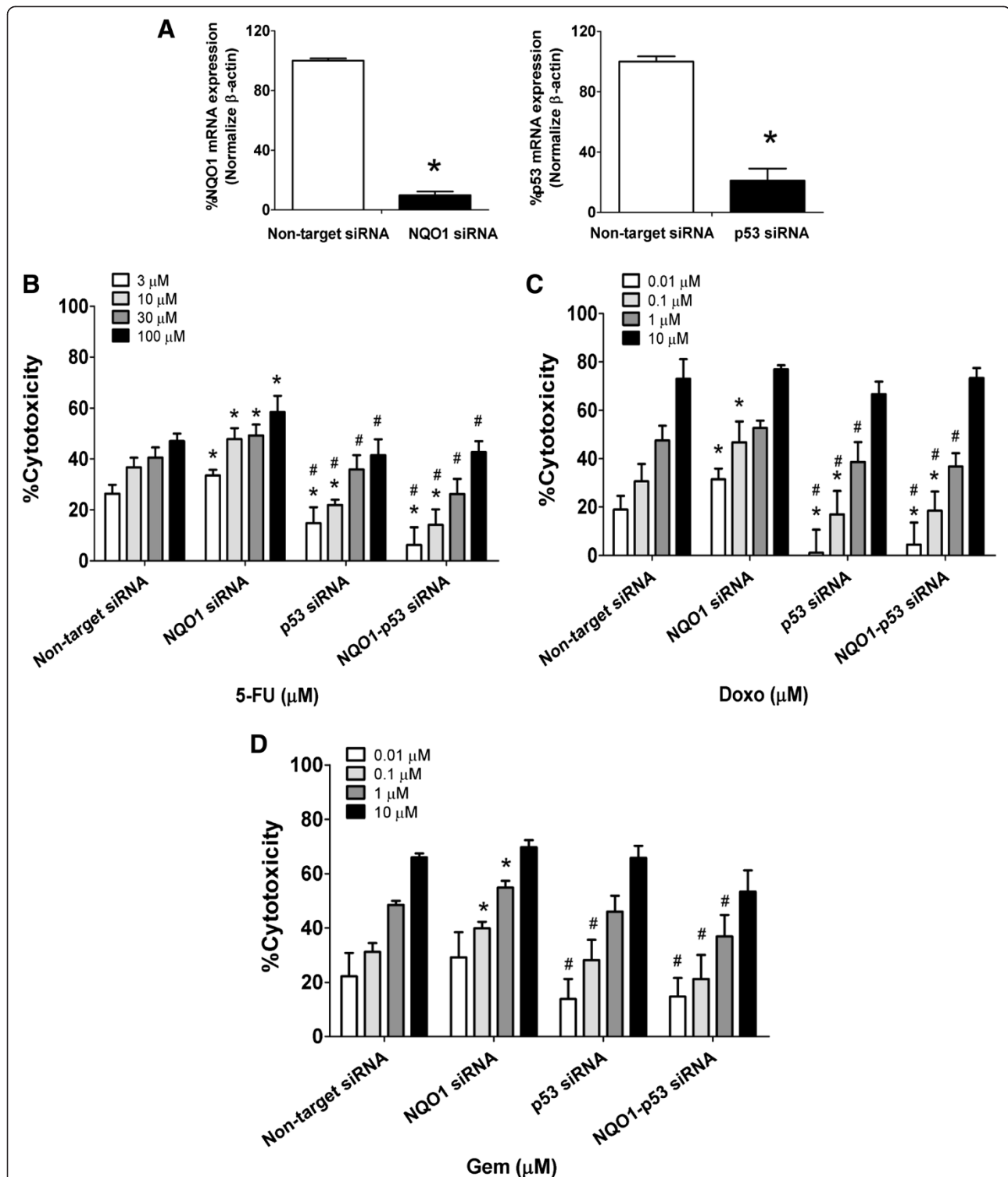
Figure 6 Double knockdown of NQO1 and p53 by siRNA altered KKKU-100 cells to chemotherapeutic agents. (A) Effect of co-transfected NQO1 and p53 siRNA in KKKU-100 cells. Cells were transfected with the pooled siRNA against NQO1 and p53 for 24 hr. The bars represent relative expression of NQO1 and p53 normalized with β-actin as internal control. (B-D) After co-transfection, cells were treated with varied concentrations of chemotherapeutic agents; 5-FU, Doxo, and Gem for another 24 hr as described in the “Methods” section. The cytotoxicity was evaluated by SRB assay. Data represent mean ± SEM, each from three separated experiments. * p < 0.05 vs the non-targeting knocked down cells and # p < 0.05 vs NQO1 knocked down cells.
