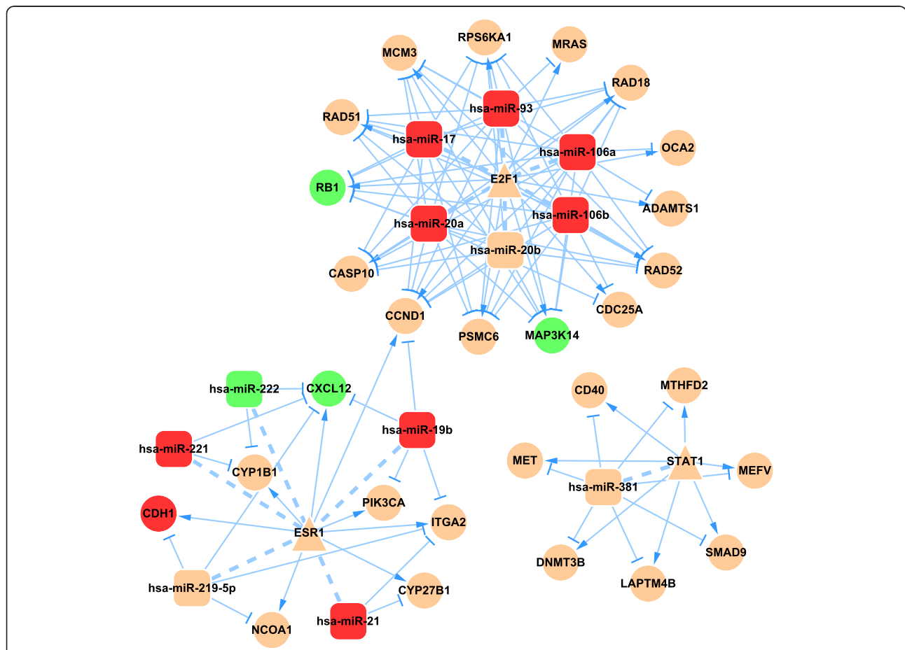
Figure 3 Lung cancer-related miRNA-TF synergistic regulatory subnetwork I. The ellipse nodes are the genes; the round rectangle nodes are the miRNAs; and the triangle nodes are the TFs. Green nodes: down-regulated nodes; red nodes: up-regulated nodes; arrow shape edge: transcriptional activation/repression; T-shape edge: miRNA repression; and dash line: a feedback loop.
