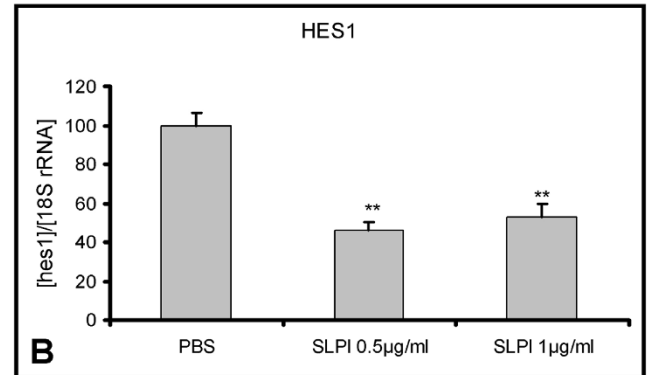
Figure 10 SLPI prevents TNF \alpha -induced I \kappa B \alpha degradation and suppresses HES1. A: Western Blot for I \kappa B \alpha with protein extracts from neural stem cells stimulated for the indicated periods with 10 ng/ml TNF \alpha with (+) or without (-) 500 ng/ml SLPI. Presentation of one of two experiments. B: Real-Time-PCR assessment of HES1 expression ( n = 3 , + std dev) in rat adult NSC after an incubation period of three days with the indicated amounts of SLPI and consecutive four days in differentiation medium. Presentation of a representative result of three experiments. *: p < 0.05 , **: p < 0.01 (according to a One Way ANOVA analysis of variance (Holm-Sidak method)).
