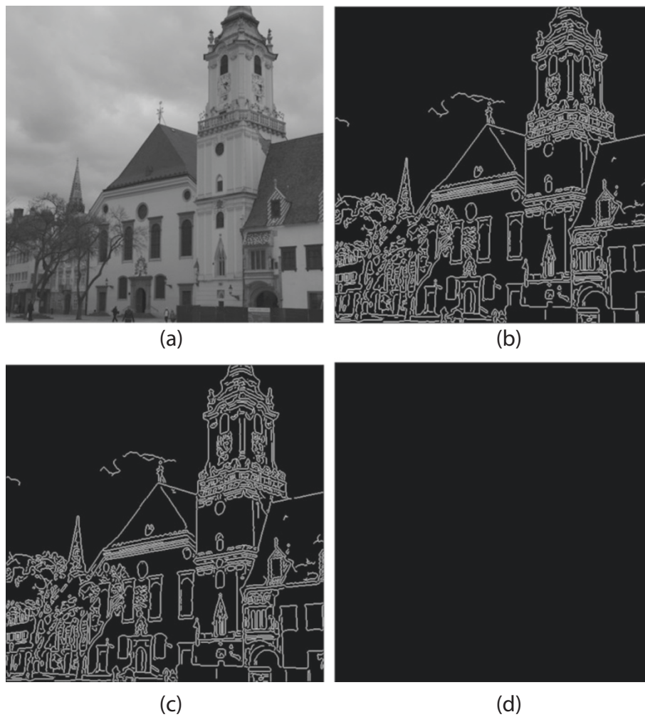
Figure 3 Change in the number of edge pixels due to embedding. (a) Cover image. (b) Edge pixels in a cover (masked). (c) Edge pixels in a stego (masked). (d) No edge pixels mismatch.
