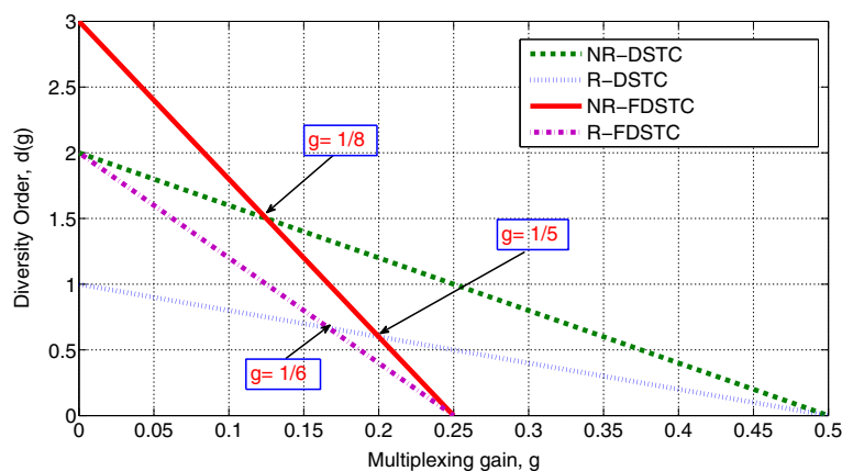
Figure 8 Diversity order d(g) versus multiplexing gain g .
