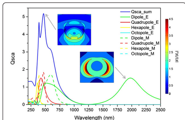
Figure 6 Scattering and near fields of a semiconductor nanoparticle. Scattering cross section of a 170 nm radius nanoparticle from GZO (refractive index data fitted with parameters from [27]) and near field distribution of the electromagnetic field around the nanoparticle for the quadrupole magnetic mode at 468 nm and the dipole electric mode at 1,978 nm as insets (incident light from the top).
