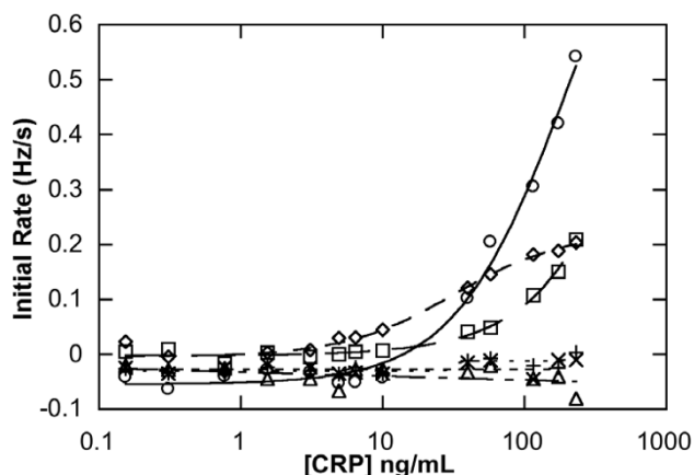
Figure 2 Three different CRP assay formats carried out using RAP showing both test channel (immobilised Sheep anti-CRP as capture antibody channels) and control channel (immobilised Sheep immunoglobulin G). Key: homogenous sandwich test channel (○); direct capture assay test channel (□); direct sandwich test channel (◇); homogenous sandwich control channel (x); direct capture control channel (+); direct sandwich control channel (Δ).
