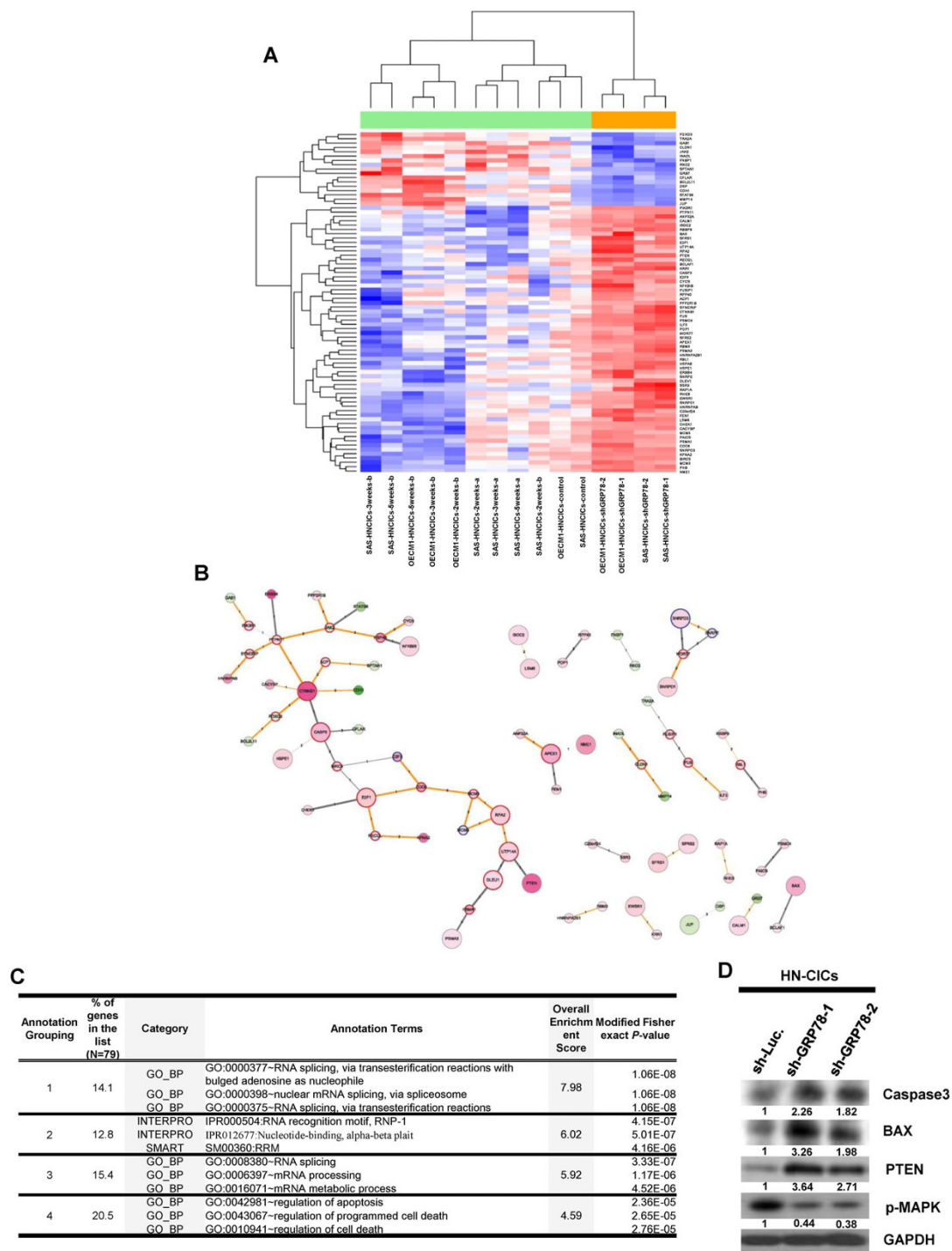
Figure 6 Differentially expressed genes in GRP78-knockdown HN-CICs. (A) A total of 79 significantly differentially expressed genes mapped in the human PPIs were clustered (by row) according to their similarities in GRP78-knockdown HN-CICs, red indicating induction and blue indicating repression. (B) Mapped human PPIs among the differentially expressed genes were grouped according to the topological characteristics as highlighted in border colors (periphery: gray; inter-modular hubs: red; and intra-modular hubs: blue). Color legends were according to expression patterns: as for nodes, red - induction and green - repression; as for edges, gray -negatively correlated and orange-positively correlated. Thickness of edges was proportional to the absolute value of PCC and numbers indicated databases reporting such interactions. (C) Top 4 functional annotation clusters analyzed from DAVID were listed. (D) Total proteins were prepared from Sh-Luc and Sh-GRP78 expressing HN-CICs and analyzed by immunoblotting with antibodies against Caspase-3, BAX, PTEN, MAPK or GAPDH as indicated. The amount of GAPDH protein of different crude cell extracts was referred as loading control.
