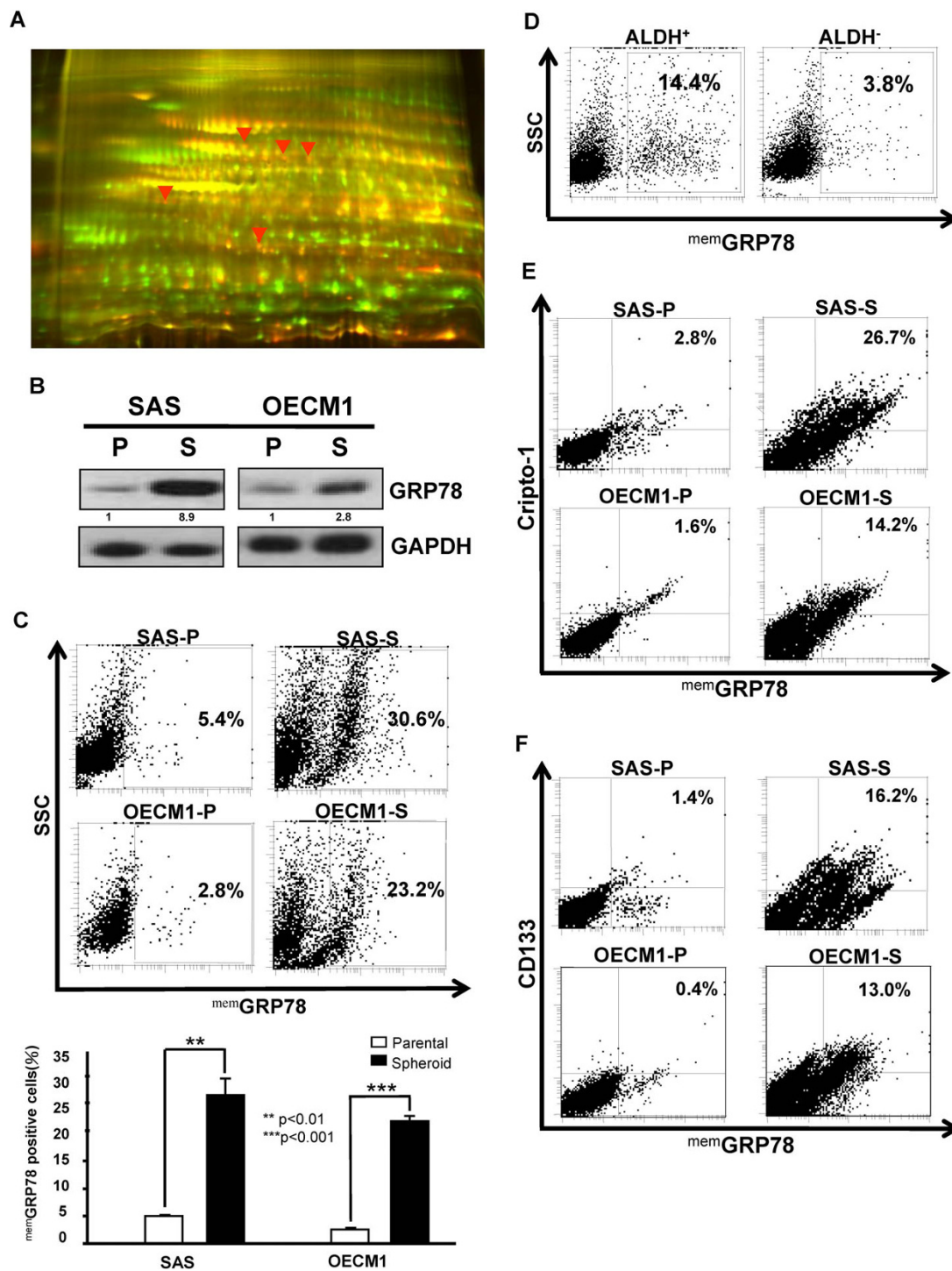
Figure 1 The differential expression of GRP78 and membrane associated GRP78 ( ^{mem}GRP78 ) in parental HNSCCs and HN-CICs. (A) The whole cell proteomes of SAS cells (Cy3-labeled, green) and SAS-derived sphere cells (HN-CICs) (Cy5-labeled, red) were collected and analyzed by two-dimensional differential gel electrophoresis (2-D DIGE). Image overlay of Cy3- and Cy5-labeled proteomes, red arrow indicates interests of up-regulated. (B) Total proteins were prepared from parental HNSCCs (SAS and OECM1) or HN-CICs (SAS and OECM1-derived spheres) and analyzed by immunoblotting with anti-GRP78 or anti-GAPDH antibodies as indicated. The amount of GAPDH protein of different crude cell extracts was referred as loading control. (C) ^{mem}GRP78 positive cells expression in HNSCCs and HN-CICs was detected by FACS (**, p < 0.01 ; ***, p < 0.001 ). (D) The percentage of ^{mem}GRP78 positive cells in isolated ALDH + and ALDH - HNSCCs, respectively. The co-expression profile between ^{mem}GRP78 and Cripto-1 (E) or CD133 (F) in HNSCCs and HN-CICs was examined by FACS. (P: Parental HNSCCs; S: HNSCCs-isolated sphere cells).
