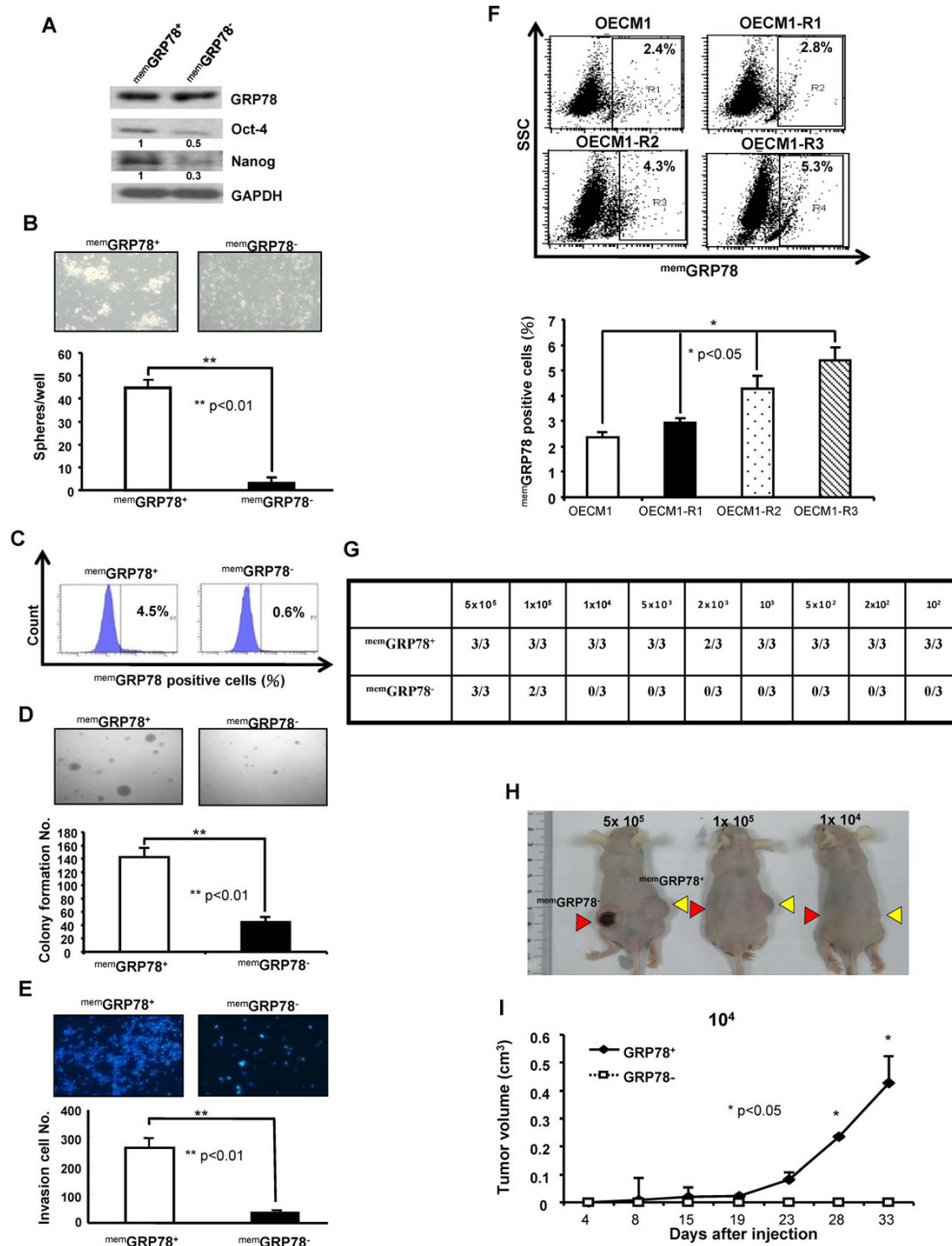
Figure 2 Cancer stem cells properties of memGRP78 + and memGRP78 - HNSCCs in vitro and in vivo. (A) Expressions of pluripotent stemness genes (Oct4 and Nanog) in memGRP78 + and memGRP78 - HNSCCs were determined by western analysis. The amount of GAPDH was referred as loading control. (B) Representative images of tumorsphere-forming ability in memGRP78 + and memGRP78 - HNSCCs grown under defined serum-free selection medium as described at Materials and Methods. The numbers of spheres were further calculated using microscope. Results are means ± SD from three experiments. (**, p < 0.01) (C) Sorted memGRP78 + and memGRP78 - cells were further cultivated with standard medium containing 10% serum. At day 10, the percentage of memGRP78 expression was re-analyzed by flow cytometry. (D) To elucidate the anchorage independent growth, single cells suspension of memGRP78 + and memGRP78 - cells plated onto soft agar and analyzed. Results are means ± SD of triplicate samples from three experiments (**, p < 0.01) (E) Invasion ability of memGRP78 + and memGRP78 - cells were plated onto transwell coated with matrigel and analyzed. Results are means ± SD of triplicate samples from three experiments (**, p < 0.01) (F) Increased radio-resistance properties (OECM1-R3 > OECM1-R2 > OECM1-R1 > parental OECM1) positively correlates memGRP78 expression in HNSCCs by FACS analysis. (*, p < 0.05) (G) Summary of the in vivo tumor growth ability of different numbers of memGRP78 + and memGRP78 - cells examined by xenotransplantation analysis. (H) Representative tumor growth of memGRP78 + and memGRP78 - HNSCCs was generated in the subcutaneous space of recipient nude mice (Yellow arrows: memGRP78 + HNSCCs; Red arrows: memGRP78 - HNSCCs). (I) Tumor volume was measured after inoculation of memGRP78 + and memGRP78 - HNSCCs in nude mice. Error bars correspond to SD (lower panel). (*, p < 0.05).
