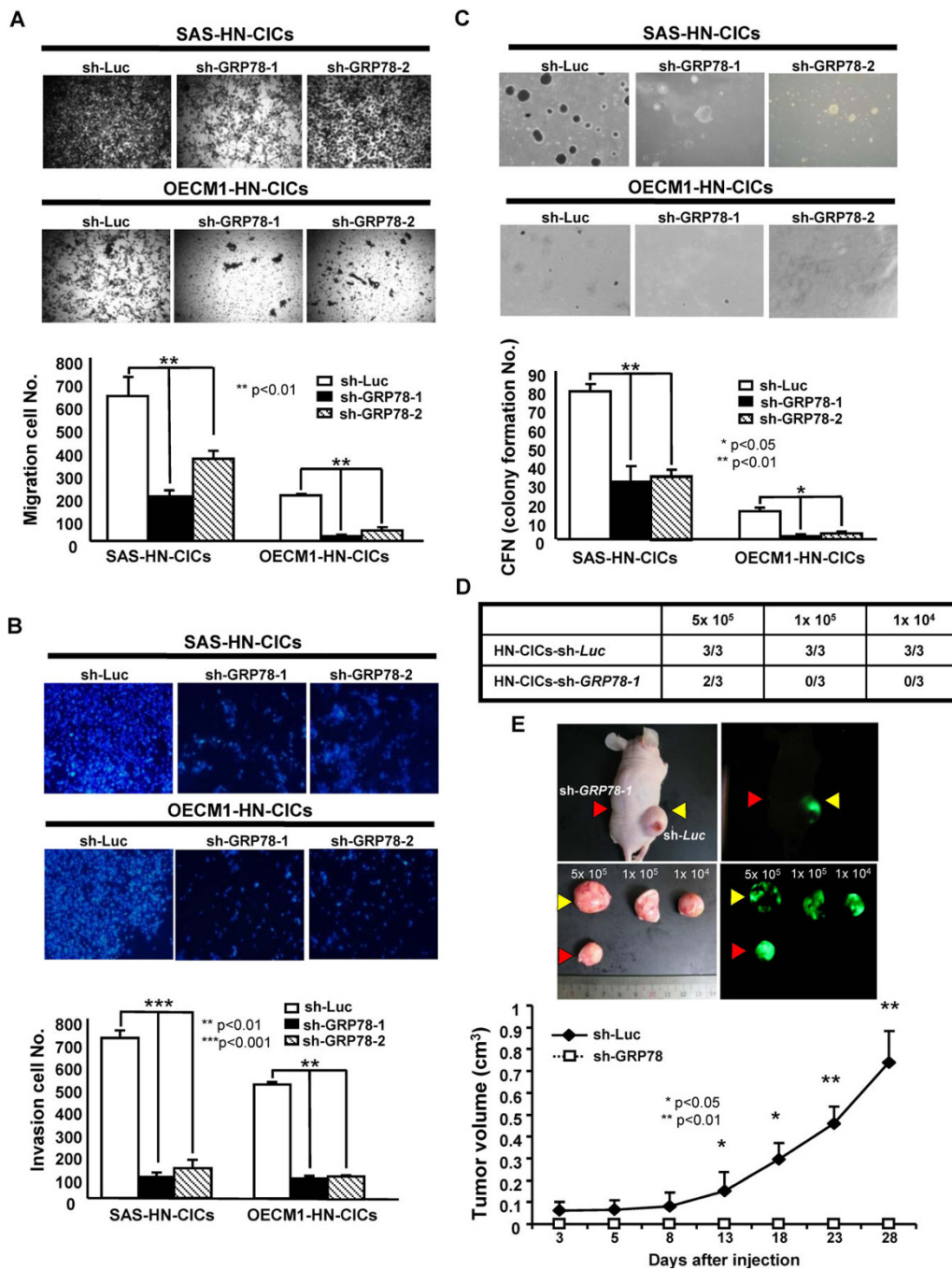
Figure 4 GRP78 inhibition impaired in vitro and in vivo tumorigenic properties of HN-CICs. (A) To elucidate the capability of migration of GRP78 shRNA knockdown and sh-Luc HN-CICs, single cell suspension of GRP78-specific shRNA or control sh-Luc HN-CICs were plated onto transwell and analyzed as described in Materials and Methods. Results are means \pm SD of triplicate samples from three experiments (**, p < 0.01 ). (B) Single cell suspension of GRP78-specific shRNA or control sh-Luc HN-CICs were plated onto transwell coated with matrigel and analyzed as described in Materials and Methods. Data are means \pm SD of triplicate samples from three experiments (**, p < 0.01 ; ***, p < 0.001 ). (C) To elucidate the anchorage independent growth, single cell suspension of stable GRP78-specific shRNA or control sh-Luc HN-CICs (SAS (upper panel), OECM1 (lower panel)) were plated onto soft agar and analyzed as described in Materials and Methods. Results are means \pm SD of triplicate samples from three experiments (*, p < 0.05 ; **, p < 0.01 ). (D) Summary of the in vivo tumor growth ability of different numbers of GRP78-knockdown or control (sh-Luc) HN-CICs examined by xenotransplantation analysis. (E) Representative tumor growth of 10000 control and 10000 GRP78-knockdown HN-CICs was generated in the subcutaneous space of recipient mice (upper panels). Tumor volume was measured after inoculation of GRP78-knockdown shRNA and sh-Luc-expressing HN-CICs (Yellow arrows: sh-Luc-expressing HNSCCs; Red arrows: sh-GRP78-expressing HNSCCs) (lower panel). Error bars correspond to SD (*, p < 0.05 ; **, p < 0.01 ).
