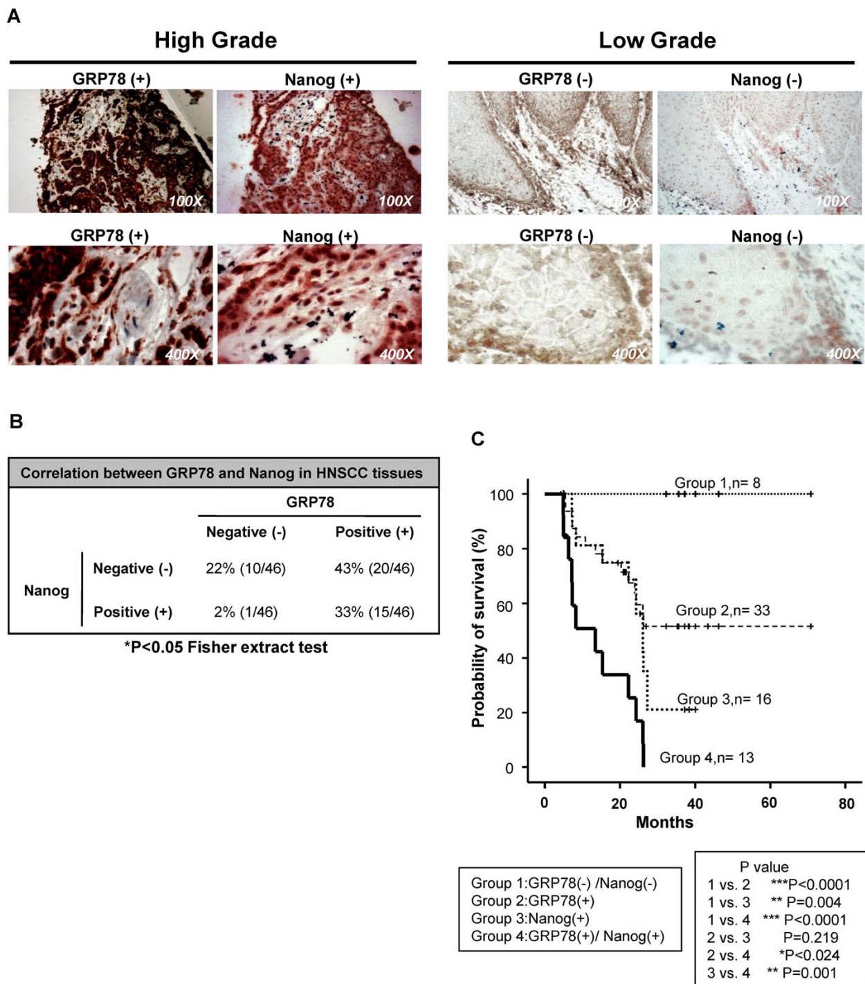
Figure 5 Co-expression of GRP78 and Nanog in HNSCC tissues. (A) Representative pictures of double positive (left panel) and double negative (right panel) in 46 HNSCC patient cases. Magnification was shown at lower right corner. (B) Statistical analysis of correlation between GRP78 and Nanog by Fisher extraction test. (C) Kaplan-Meier analysis of overall survival in HNSCC patients according to the expression of GRP78 and Nanog (Group1: GRP78(+)/Nanog(+), Group2: GRP78(+), Group3: Nanog (+) and Group4: GRP78 (-)/Nanog(-)). (*, p < 0.05; **, p < 0.01; ***, p < 0.001).
