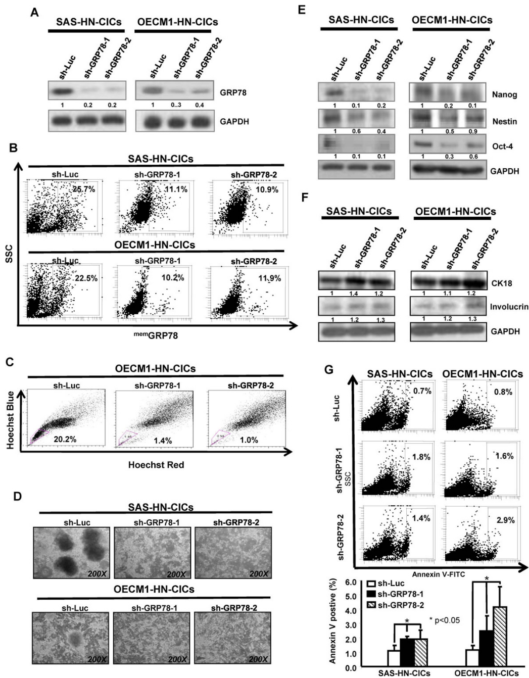
Figure 3 Suppression of GRP78/ mem GRP78 expression diminished spheres-forming capability, stemness genes expression, and side population cells of HN-CICs. (A) Down-regulation of GRP78 in HN-CICs (SAS (left panel) and OECM1 (right panel) mediated by shRNAi was validated by western blotting. (B) The percentages of mem GRP78 + cells in sh-GRP78 knockdown and sh-Luc HN-CICs were compared by flow cytometry analysis, respectively. (C) Single cell suspensions of sh-GRP78 and sh-Luc-expressing HN-CICs incubated with Hoechst 33342 were examined for side population by flow cytometry. (D) HNSCCs-enriched sphere cells were first infected with Sh-GRP78-1, Sh-GRP78-2 or Sh-Luc lentivirus, and further cultivated under the serum-free defined selection medium. The tumor sphere formation capability and cellular morphology of enriched HN-CICs (Upper panel, SAS; Lower panel; OECM1) treated with either sh-Luc or GRP78-shRNA lentivirus were examined with microscope. (E) Total proteins from figure 3d were isolated and immunoblotted by using antibodies against, anti-Oct-4, anti-Nanog, anti-Nestin or anti-GAPDH antibodies as indicated. The amount of GAPDH protein of different crude cell extracts was referred as loading control. (F) Protein level of epithelial specific differentiation markers, CK18 and involucrin in enriched HN-CICs cells infected with sh-Luc, or sh-GRP78 lentivirus was assessed by western blot. (G) Single cell suspension of spheres prepared from figure 3d transduced with sh-Luc or sh-GRP78 lentivirus were stained with Annexin V and examined by flow cytometry. The experiments were repeated three times and representative results were shown. Results are means ± SD (*, p < 0.05).
