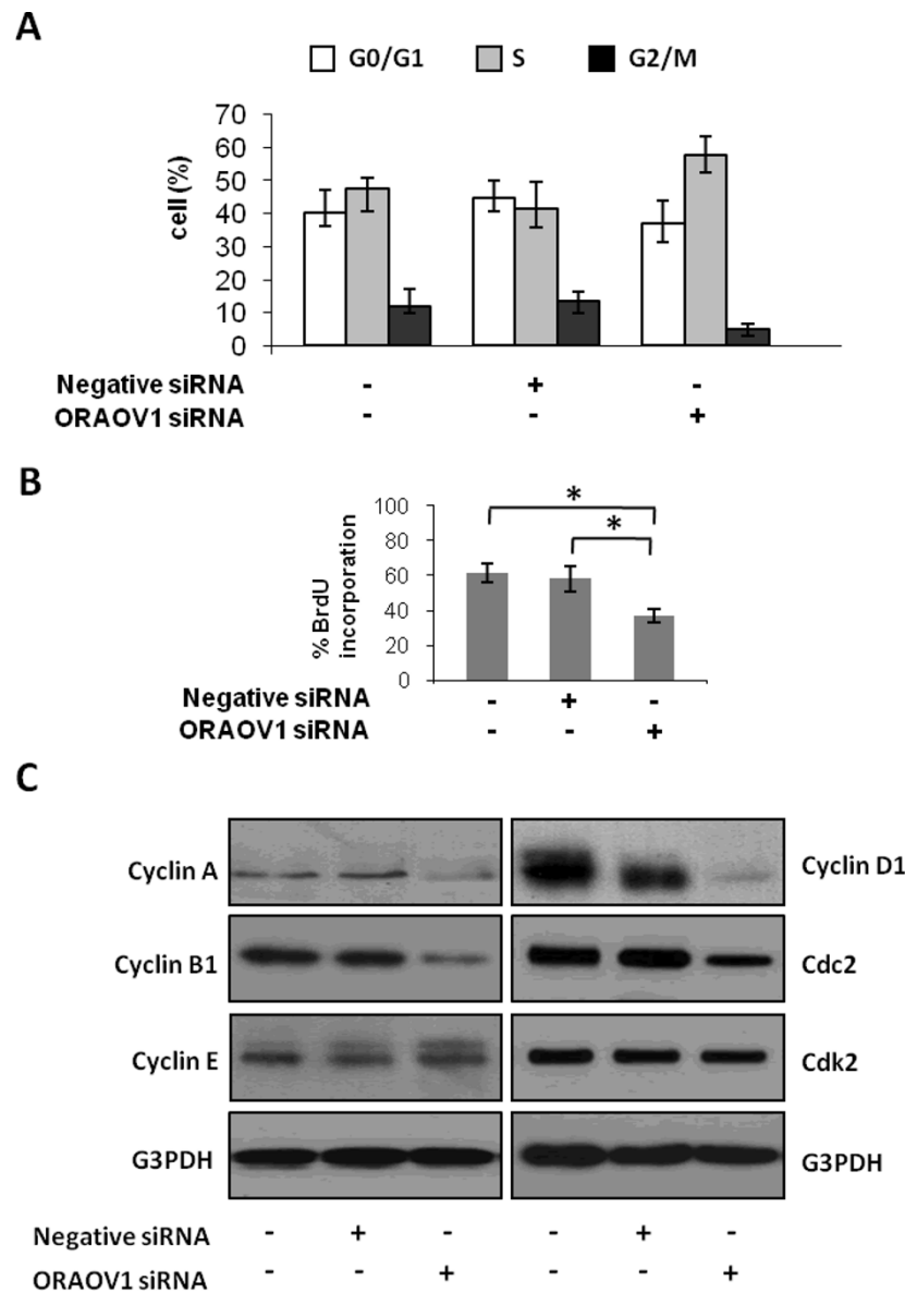
Figure 2 ORAOV1 silencing induces S-phase cell cycle arrest in HeLa cells. (A) Quantification of cell cycle distribution determined by flow cytometry analysis at 48 hours posterior to the treatment. Data were Mean \pm SE for triplicate experiments. (B) BrdU incorporation assay was performed at 48 hrs posterior to the treatment. Each column represents a mean value of triplicate experiments in each group. Data are Mean \pm SE, *, P < 0.05 . (C) Western blot analyses of the expression of Cyclin A, Cyclin B1, Cyclin E, Cyclin D1, Cdc2, and Cdk2. G3PDH was used as an internal control for equal loading. Data were representative blots from three independent experiments.
