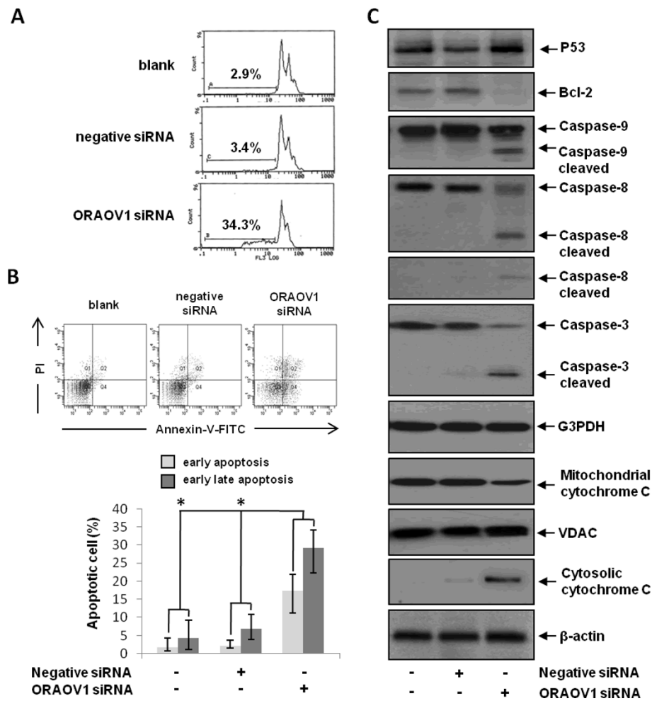
Figure 3 ORAOV1 silencing induces apoptosis in HeLa cells. (A) Analysis of HeLa cell apoptosis (sub-G1 cells) upon ORAOV1 silencing by flow cytometry assay using PI staining. (B) Quantitative analysis of cell apoptosis by Annexin V and PI double staining. Data were Mean \pm SE for triplicate experiments, * P < 0.05 . (C) The effect of ORAOV1 silencing on the expression of P53, Bcl-2, Caspase-3, 8 and 9, and cytochrome c (mitochondrial and cytosolic). G3PDH was used as an internal control for protein equal loading, and VDAC and \beta -actin was used as equal mitochondria and cytosol loading control respectively. Data was representative blots of three independent experiments.
