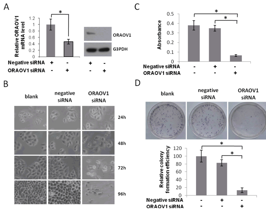
Figure 1 ORAOV1 silencing inhibits cell growth and colony formation ability in HeLa cells. (A) The expression levels of ORAOV1 mRNA and ORAOV1 protein in HeLa cells upon transfection with 100 nM ORAOV1 siRNA for 48 hrs were analyzed by real time PCR and Western blot assay respectively. 100 nM non-targeting siRNA-transfected HeLa cells and blank cells were used as controls. Results represent the means \pm SE (n = 3). *, P < 0.05 . (B) The effect of ORAOV1 silencing on HeLa cell growth. (C) Examination the effect of ORAOV1 silencing on HeLa cell proliferation by MTT assay. Results represent the means \pm SE (n = 3). *, P < 0.001 . (D) Test the effect of ORAOV1 silencing on HeLa cell colony formation ability by plate colony assay. The relative colony formation efficiency of the blank cells was set as 1. Each column represents a mean value of triplicate experiments in each group. Data are Mean \pm SE, *, P < 0.001 .
