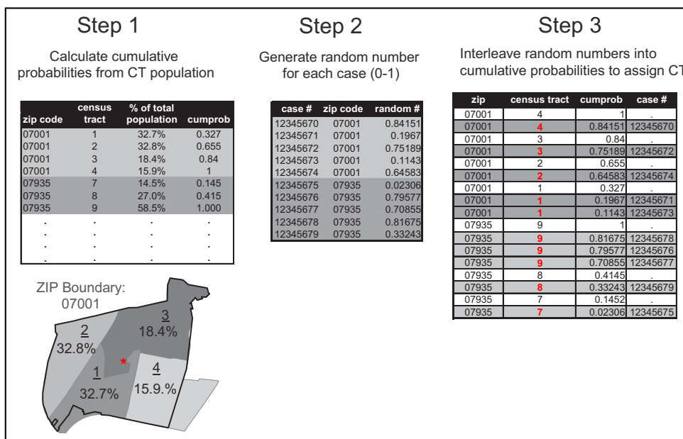
Figure 2 Procedures used for geo-imputation.
