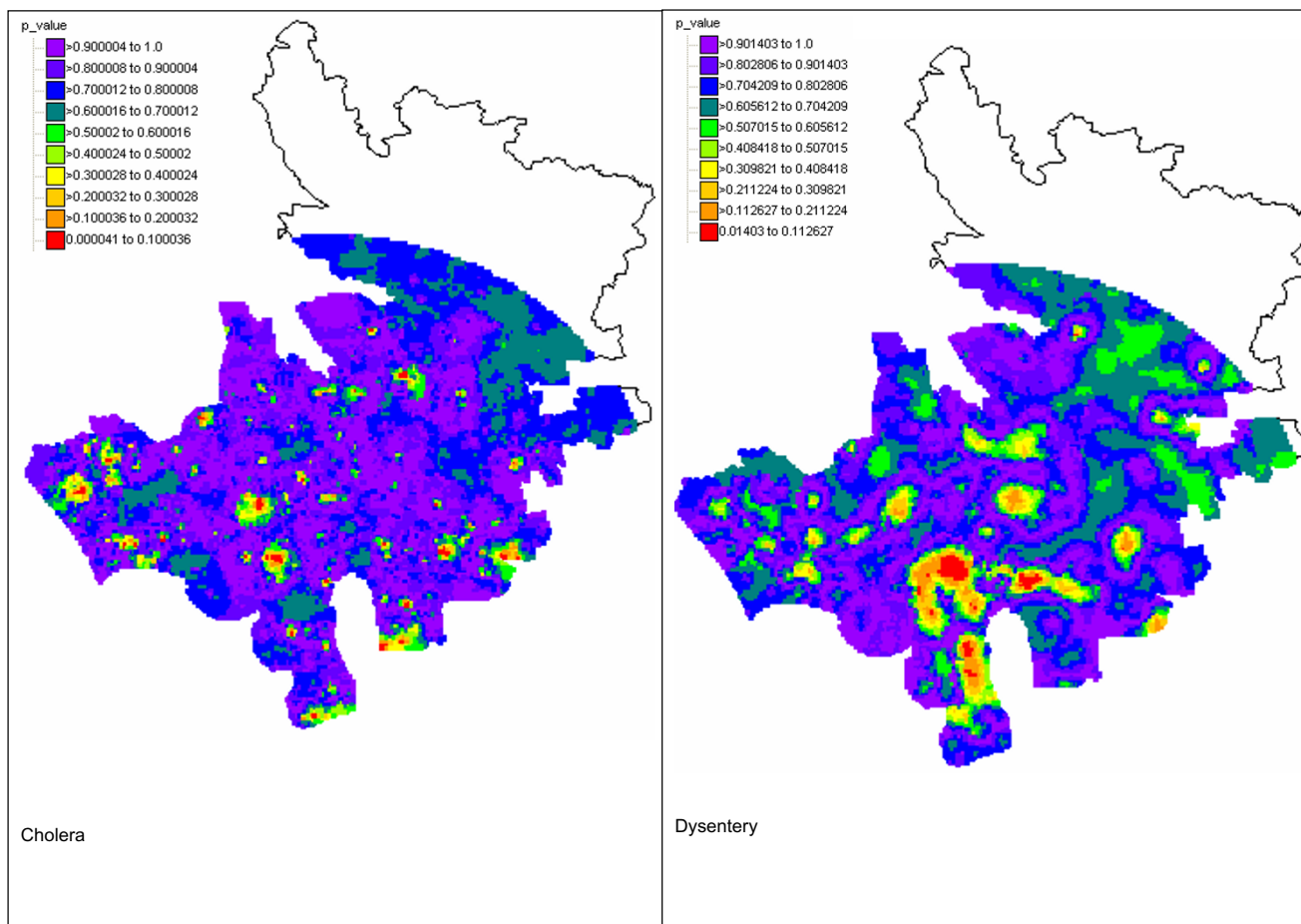
Figure 6 Maps of the p-values for the test of uniformity of local incidence rates for cholera and dysentery in Matlab 1994. At each location, the population-weighted mean of all bari rates is compared to the probability distribution of the local incidence rate which is fully characterized by the Poisson kriging estimate and variance. The lower the p-value, the more likely the local rate is significantly smaller or higher than the regional rate.
