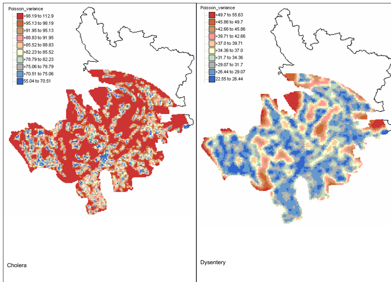
Figure 5 Maps of Poisson kriging variance for cholera and dysentery incidence risk in Matlab 1994. The class boundaries of the color legend correspond to the deciles of the histogram of kriging variances.
