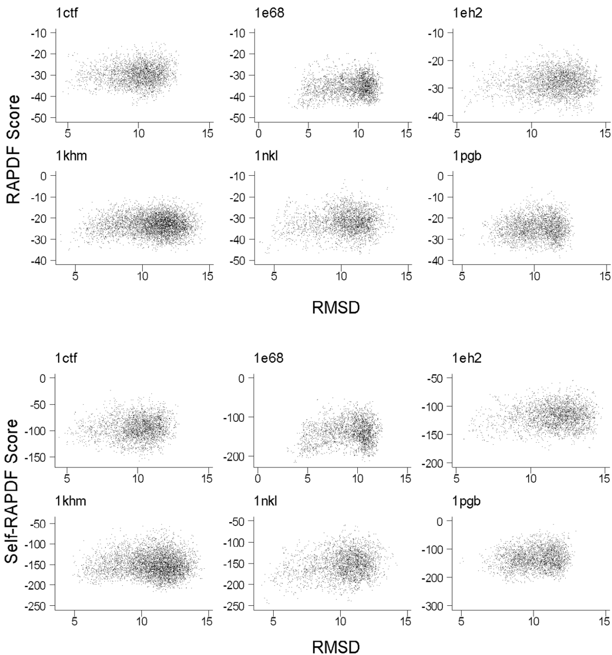
Figure 6 Scatter plot of RAPDF score or self-RAPDF score versus C_{\alpha} RMSD for six semifold decoy sets. Both RAPDF score and self-RAPDF score do not discriminate decoys well on these sets.
